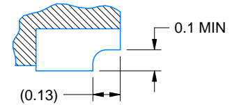
SECTION A-A TYPICAL
