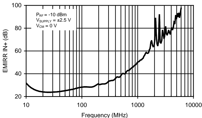
Figure 1. OPA227 EMIRR IN+ vs Frequency
