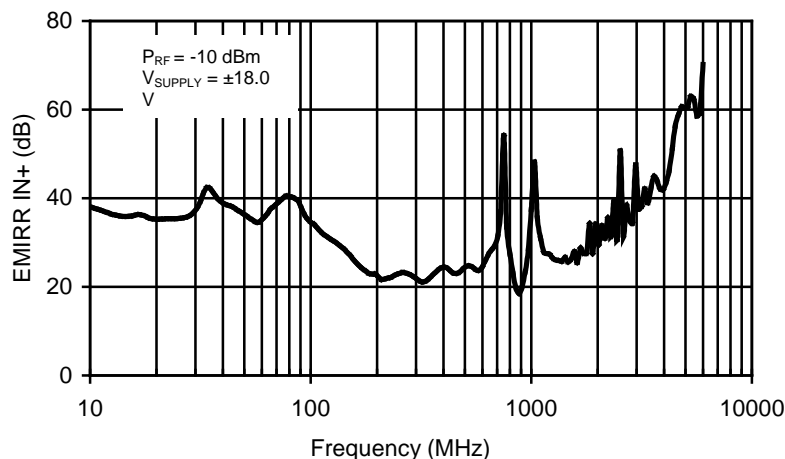
Figure 1. OPA209 EMIRR IN+ vs Frequency
