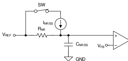
Figure 27. Simplified Soft-Start Circuit
