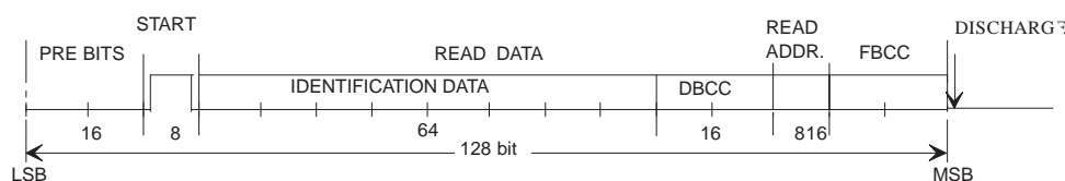
Figure 5. MPT Read Data Format
