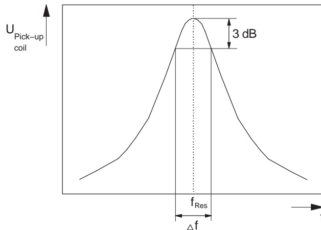
Figure 16. Determination of the Resonance Frequency and -3db Bandwidth by Monitoring the Pick-Up Coil Voltage
