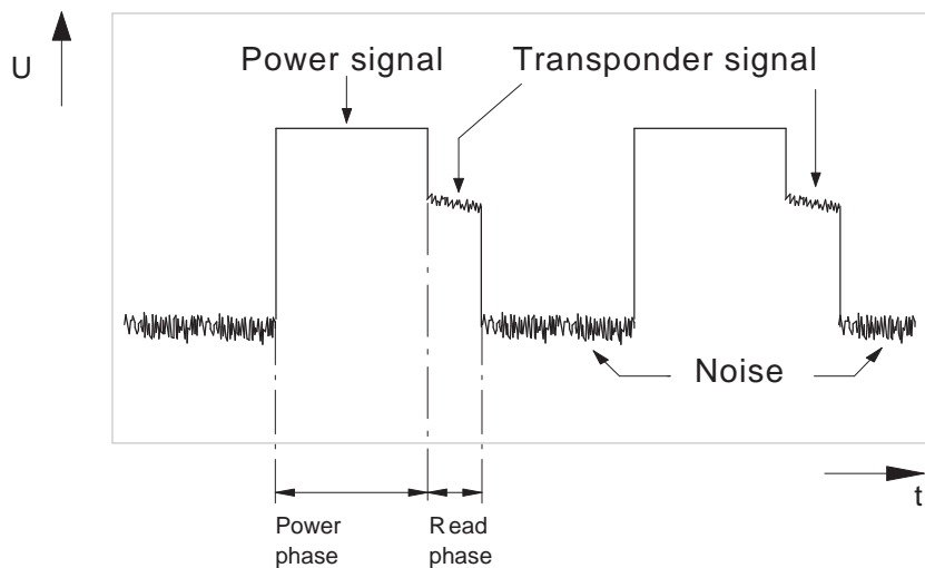
Figure 21. Monitored Signal Voltage at the Spectrum Analyser (Time Domain Mode)
