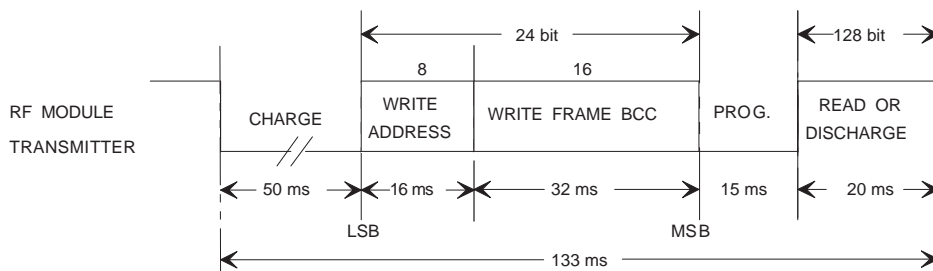
Figure 10. Data Format of the Lock Page Function
