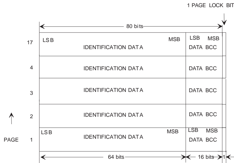
Figure 3. Memory Organisation of the MPT 0/17
