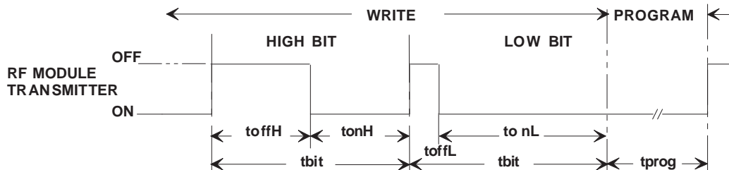
Figure 14. Write and Program Function
