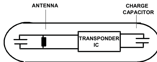
Figure 2. Block Diagram of the TIRIS Transponder
