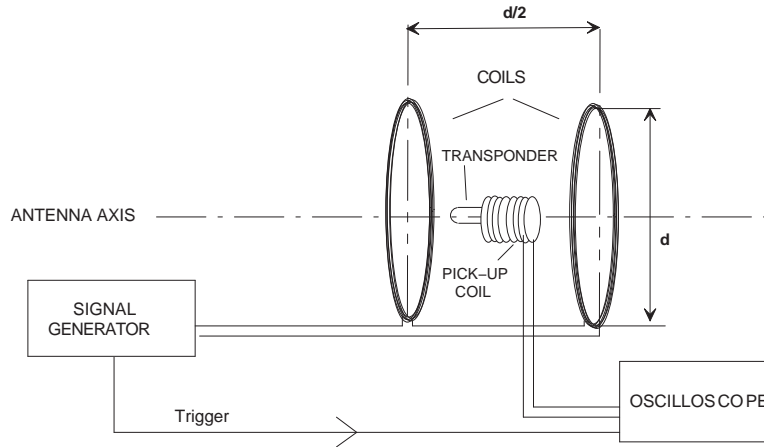
Figure 18. Test Set-up for Powering Field Strength Determination
