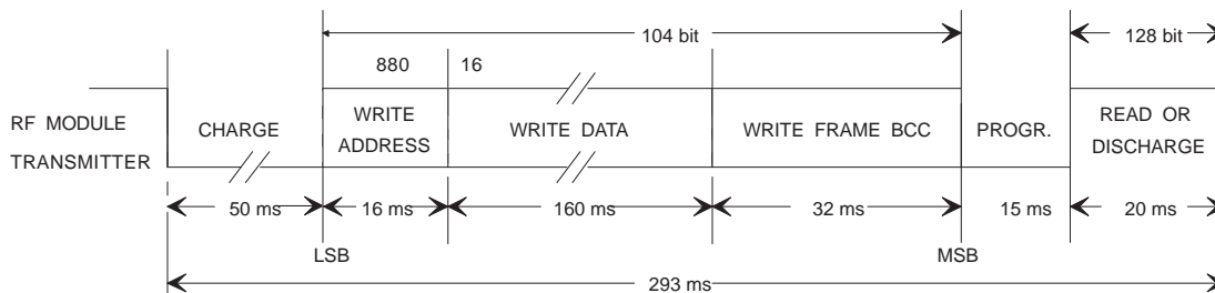
Figure 8. Data Format of the Program Page Function
