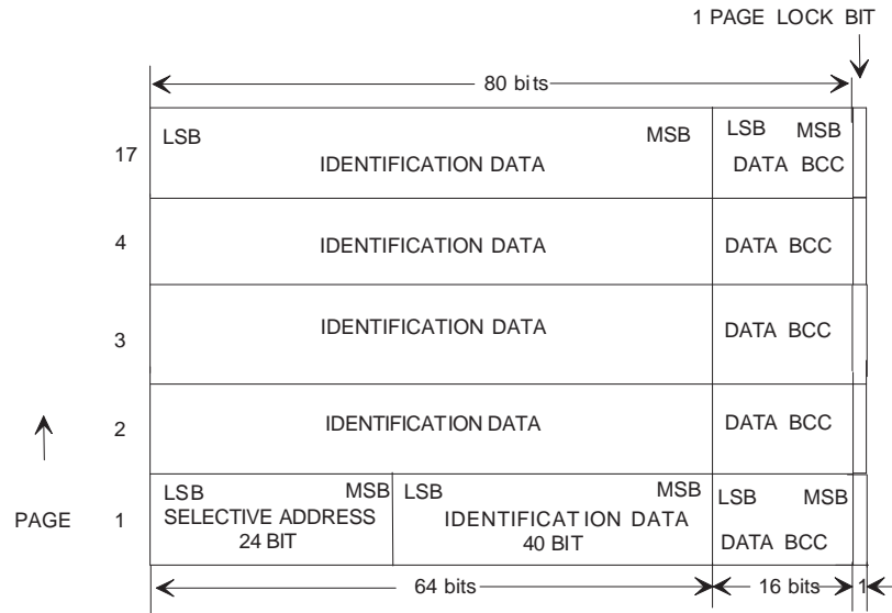
Figure 4. Memory Organisation of the SAMPT & SAMPTS 0/17-24
