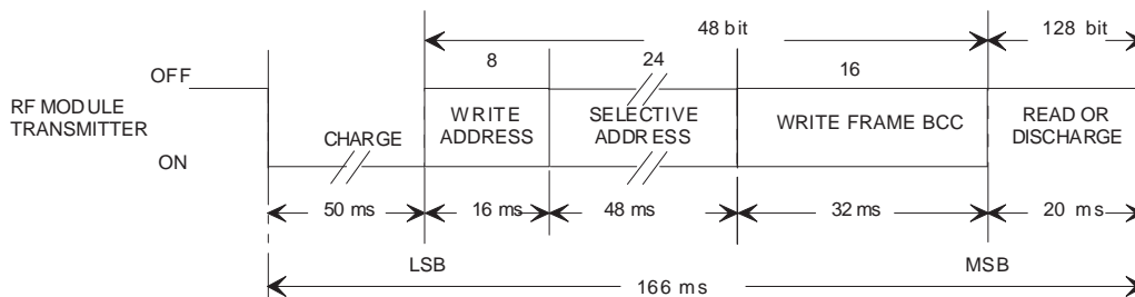
Figure 11. Data Format of the Selective Lock Page Function
