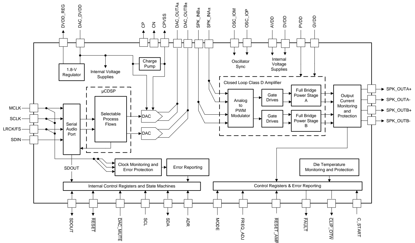
Figure 1. TAS3251 Functional Block Diagram
