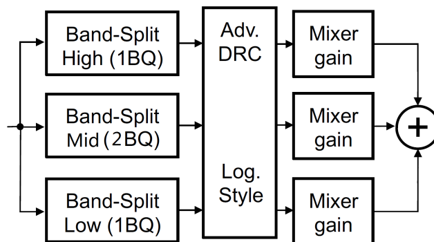
Figure 20. 3-Band DRC
