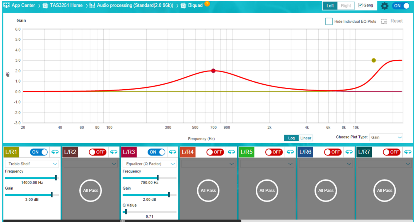
Figure 12. Equalizer Tuning Window
