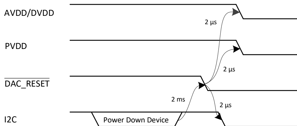
Figure 37. Power-Down Timing
