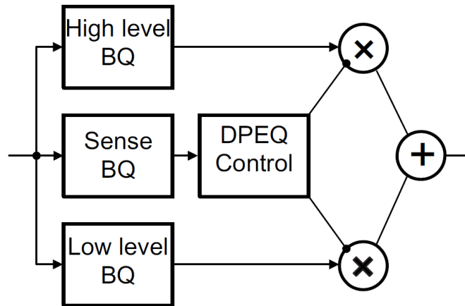
Figure 17. DPEQ
