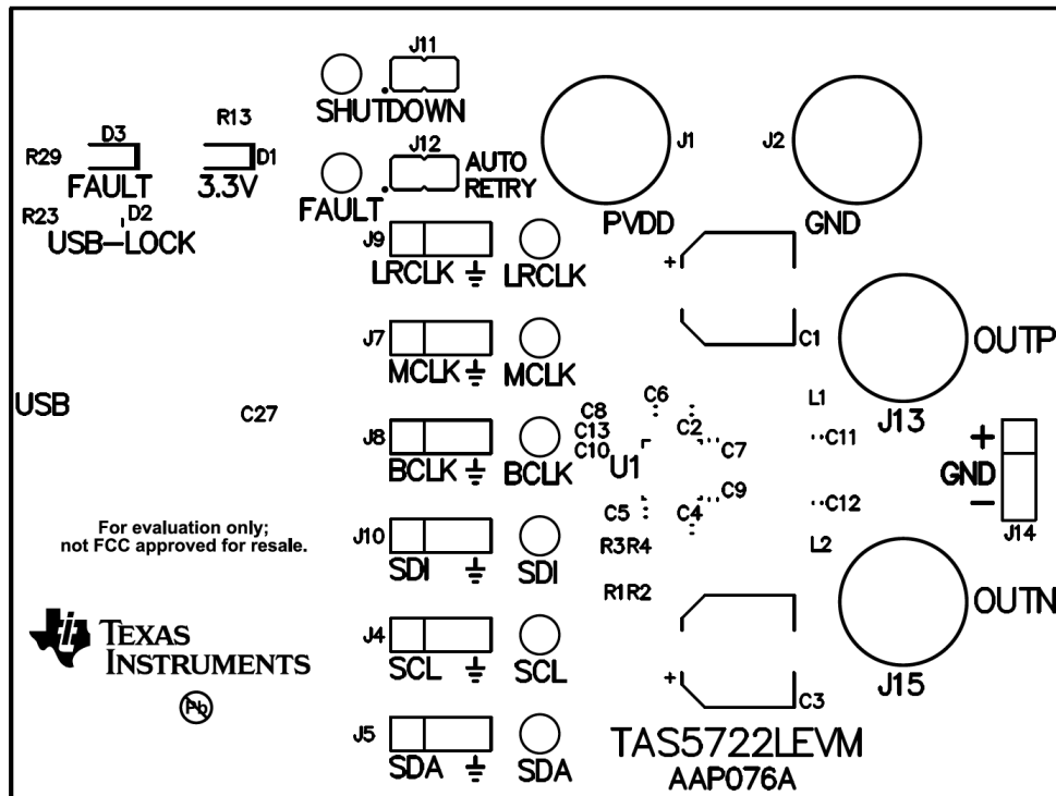
Figure 7. Top Overlay
