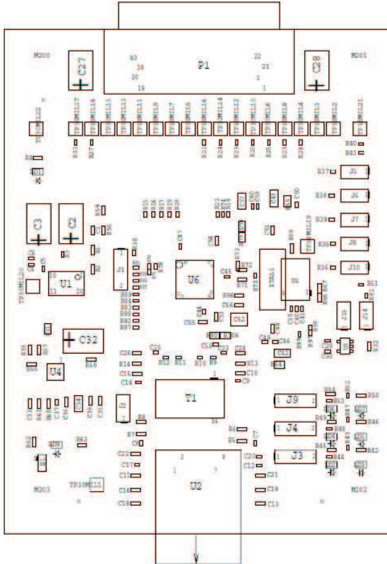
Figure 2. EVM Layout
