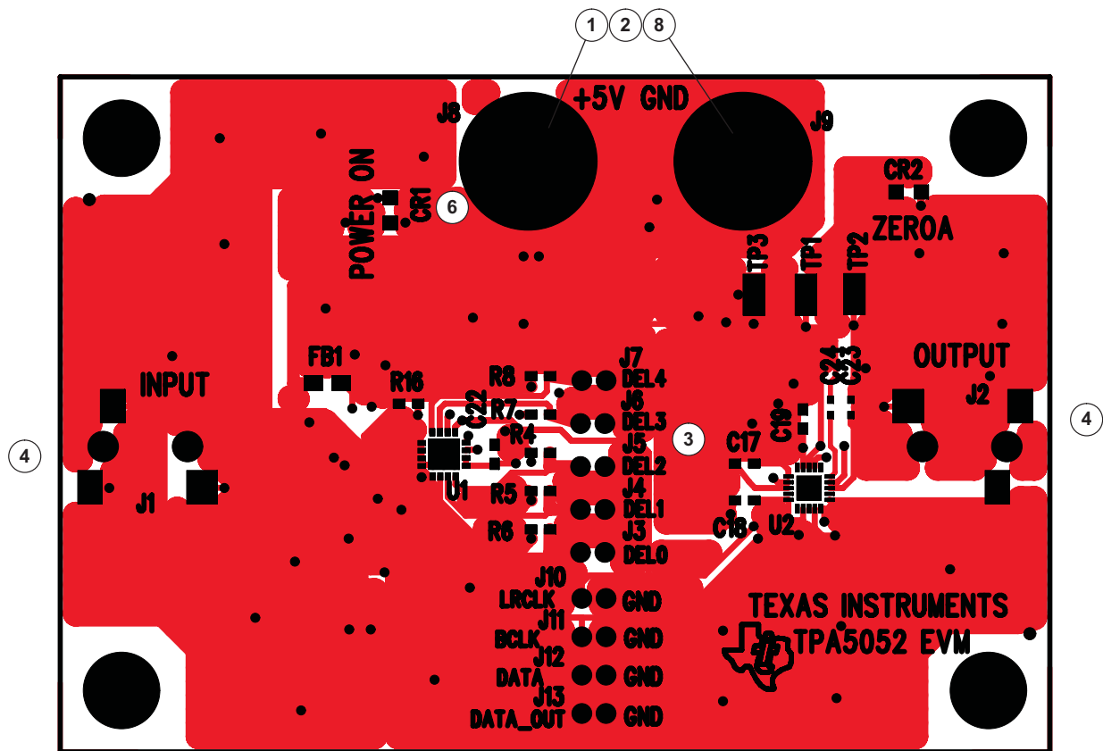
Figure 1. Top Layer of TPA5052EVM
