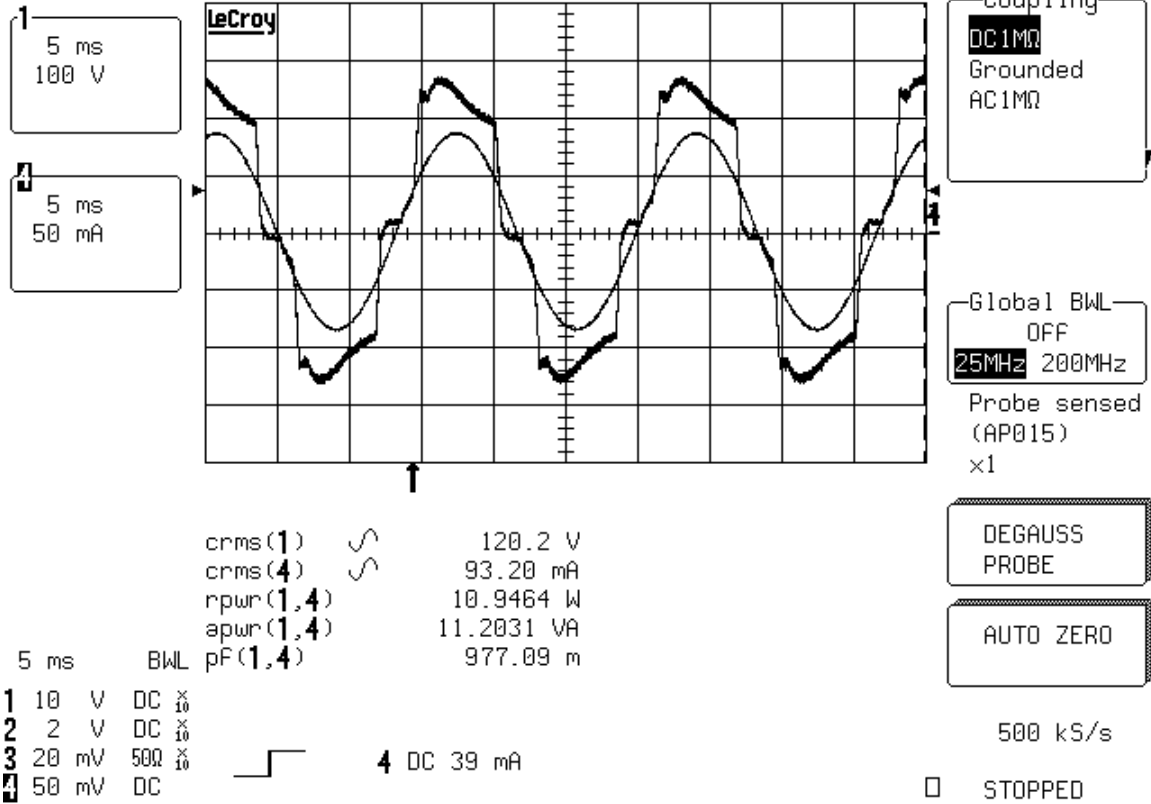
Line current and voltage
