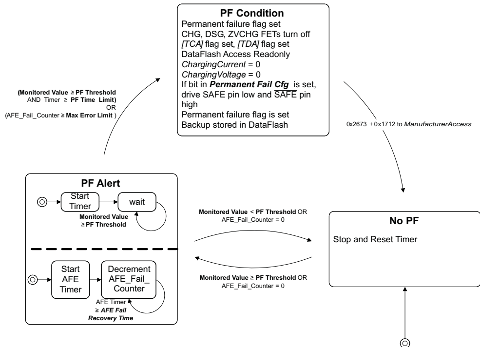
Figure 2-6. Second-Level Protection
