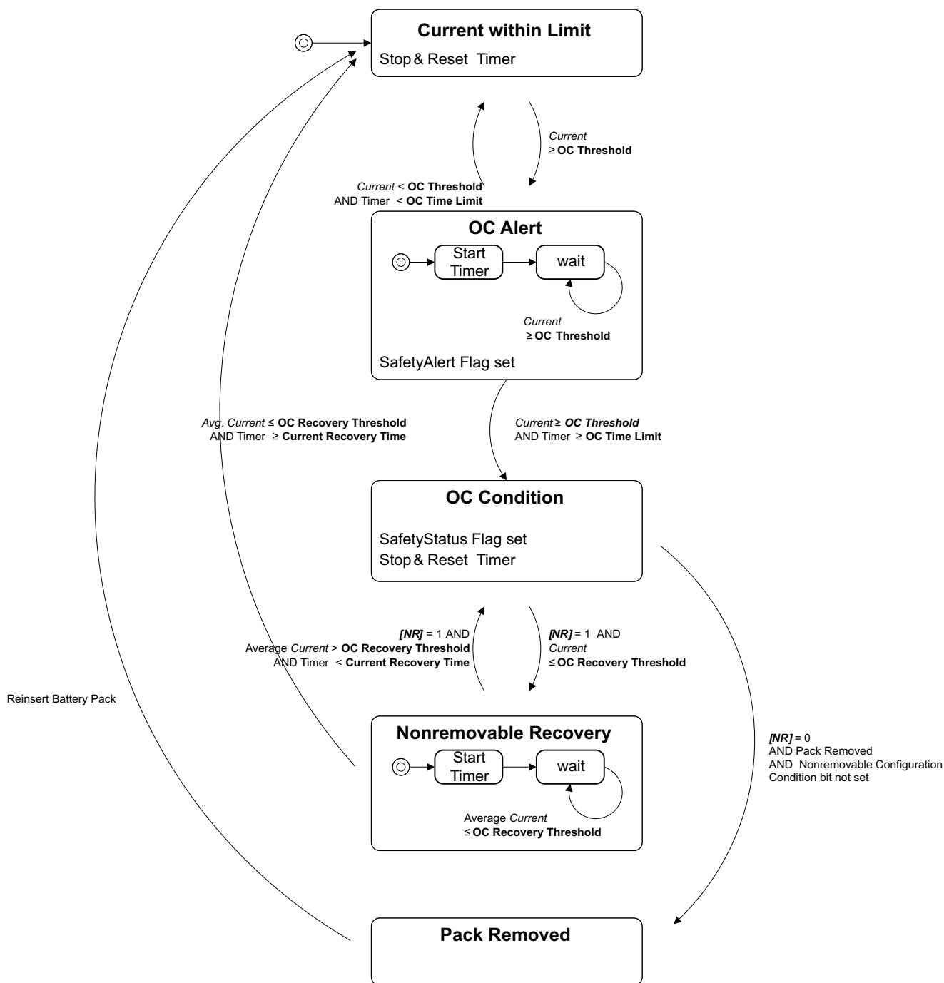
Figure 2-3. OC Protection
