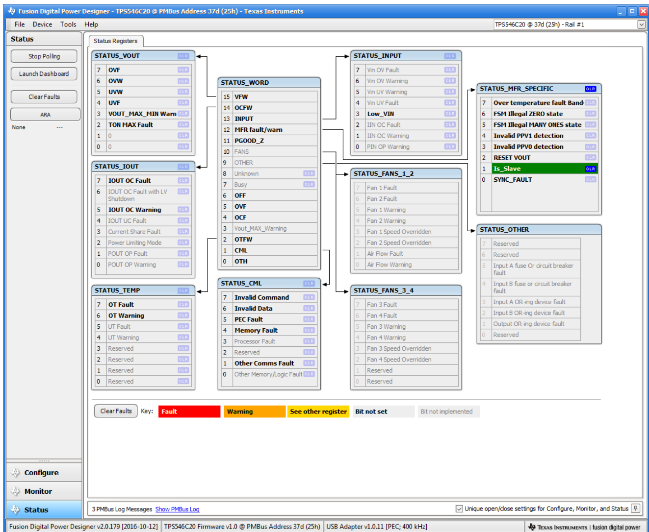
Figure 10-9. Status Screen
