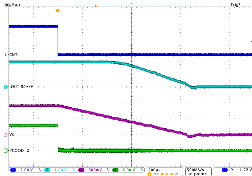
Figure 7-9. Soft Stop from Control, 0.9-V Output at 12 V_{IN} , 0-A Output
