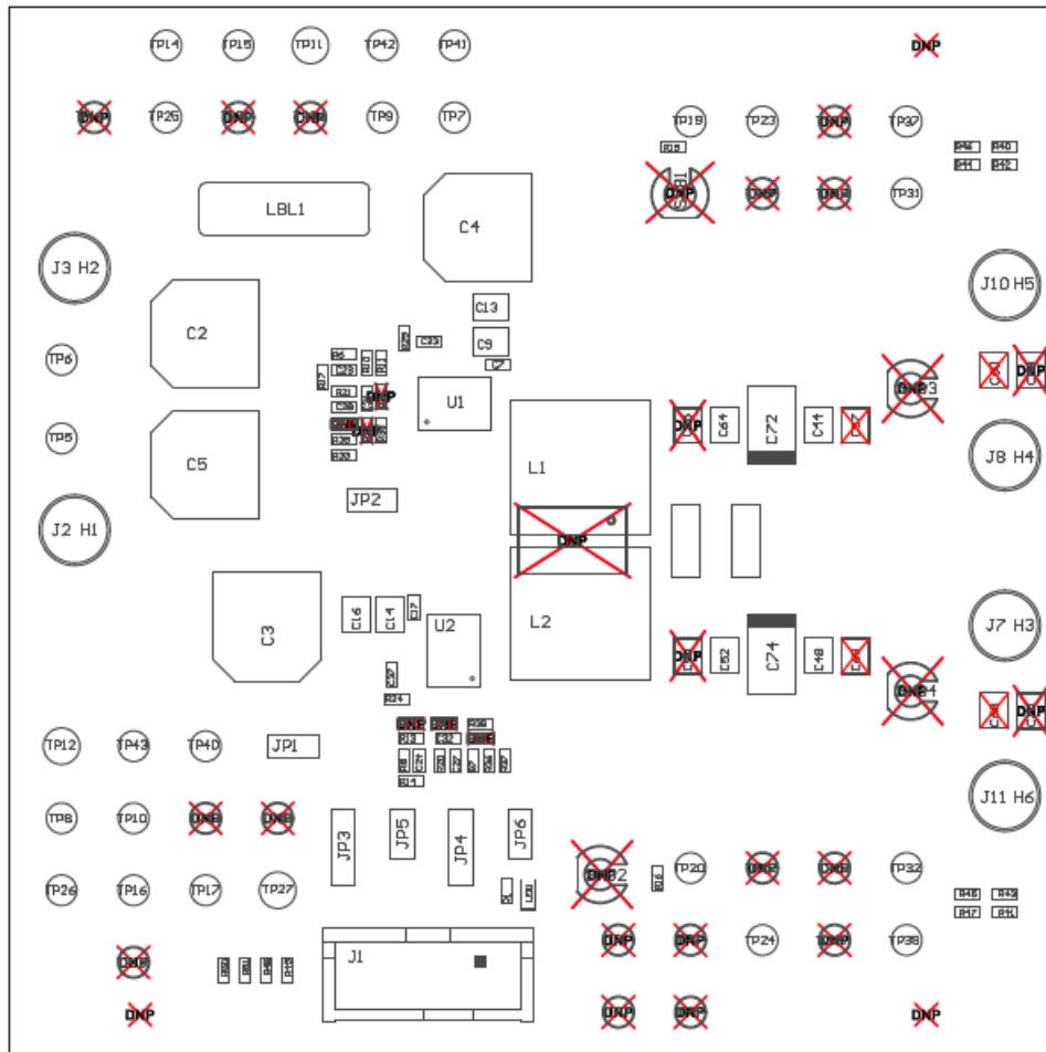
Figure 8-2. TPS546C20AEVM2-746 EVM Top Layer Assembly Drawing (Top View)
