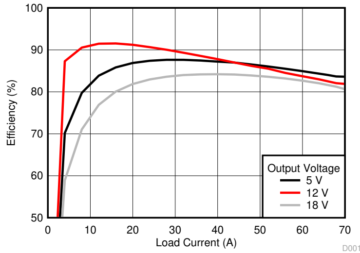
Figure 7-1. Efficiency of 0.9-V Output vs Line and Load
