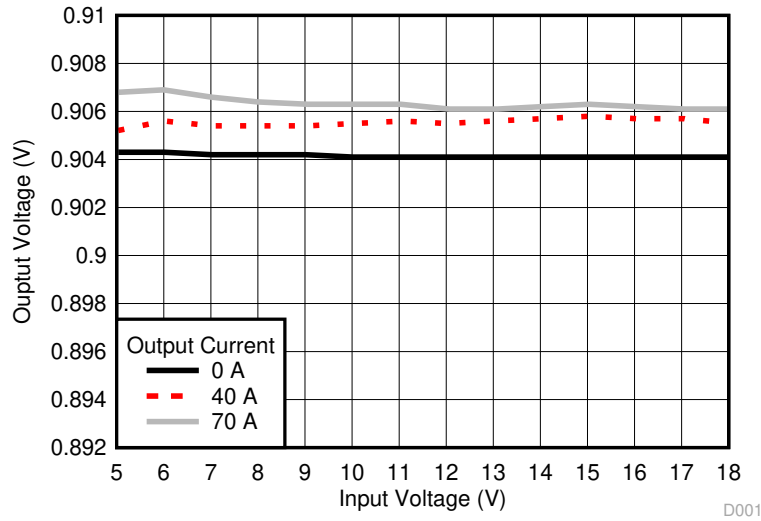
Figure 7-3. Line Regulation of 0.9-V Output (Different Board)
