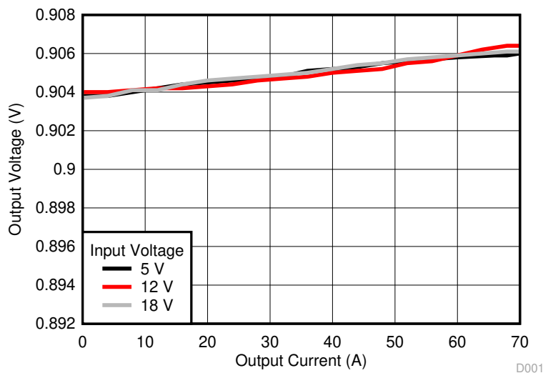
Figure 7-2. Load Regulation of 0.9-V Output
