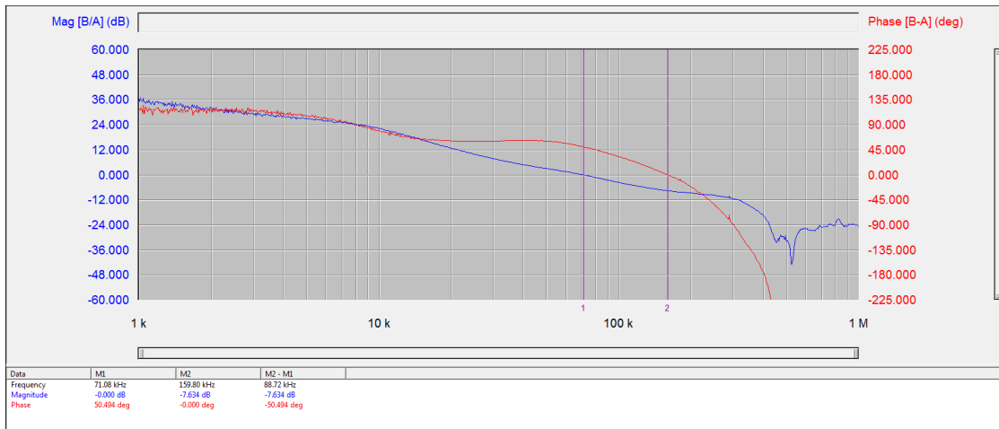
Figure 7-13. Bode Plot at 0.9-V Output at 12 V IN , 70-A Output
