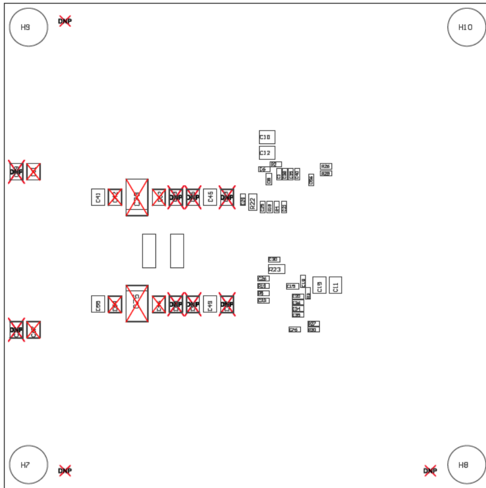
Figure 8-3. TPS546C20AEVM2-746 EVM Bottom Assembly Drawing (Bottom View)
