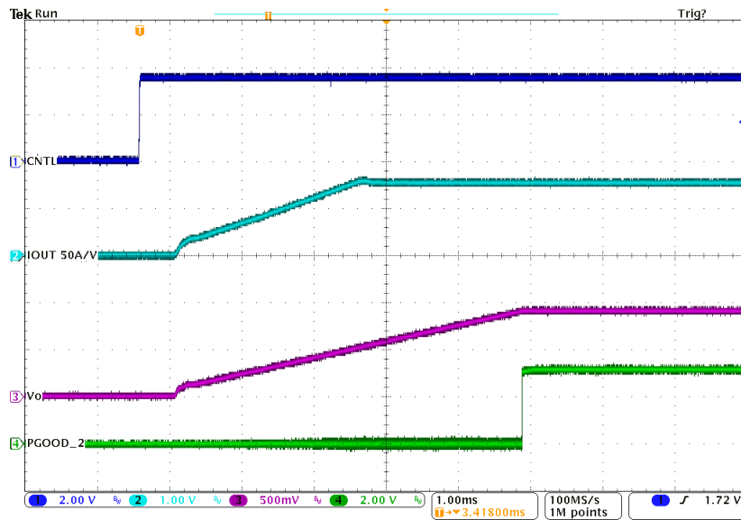
Figure 7-7. Start-Up from Control, 0.9-V Output at 12 V_{IN} , 0-A Output
