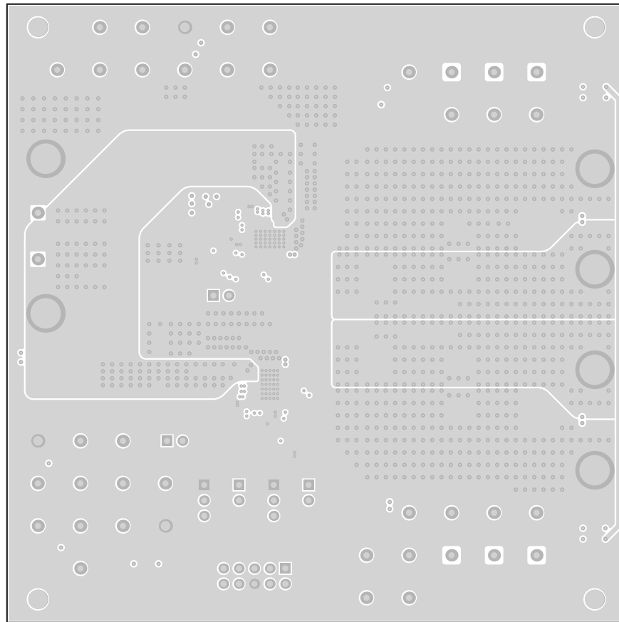
Figure 8-8. TPS546C20AEVM2-746 EVM Internal Layer 4 (Top View)
