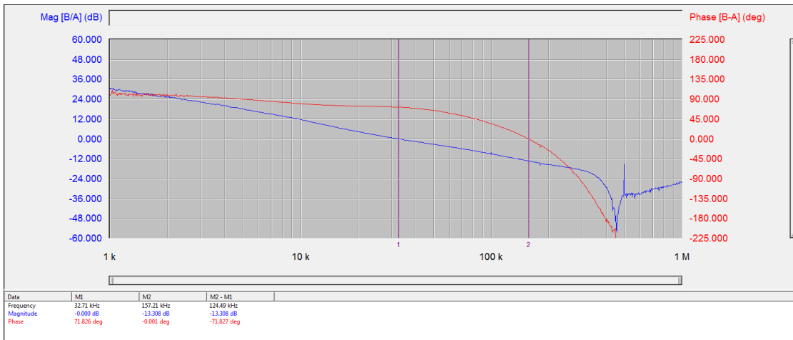
Figure 7-12. Bode Plot at 0.9-V Output at 12 V IN , 0-A Output
