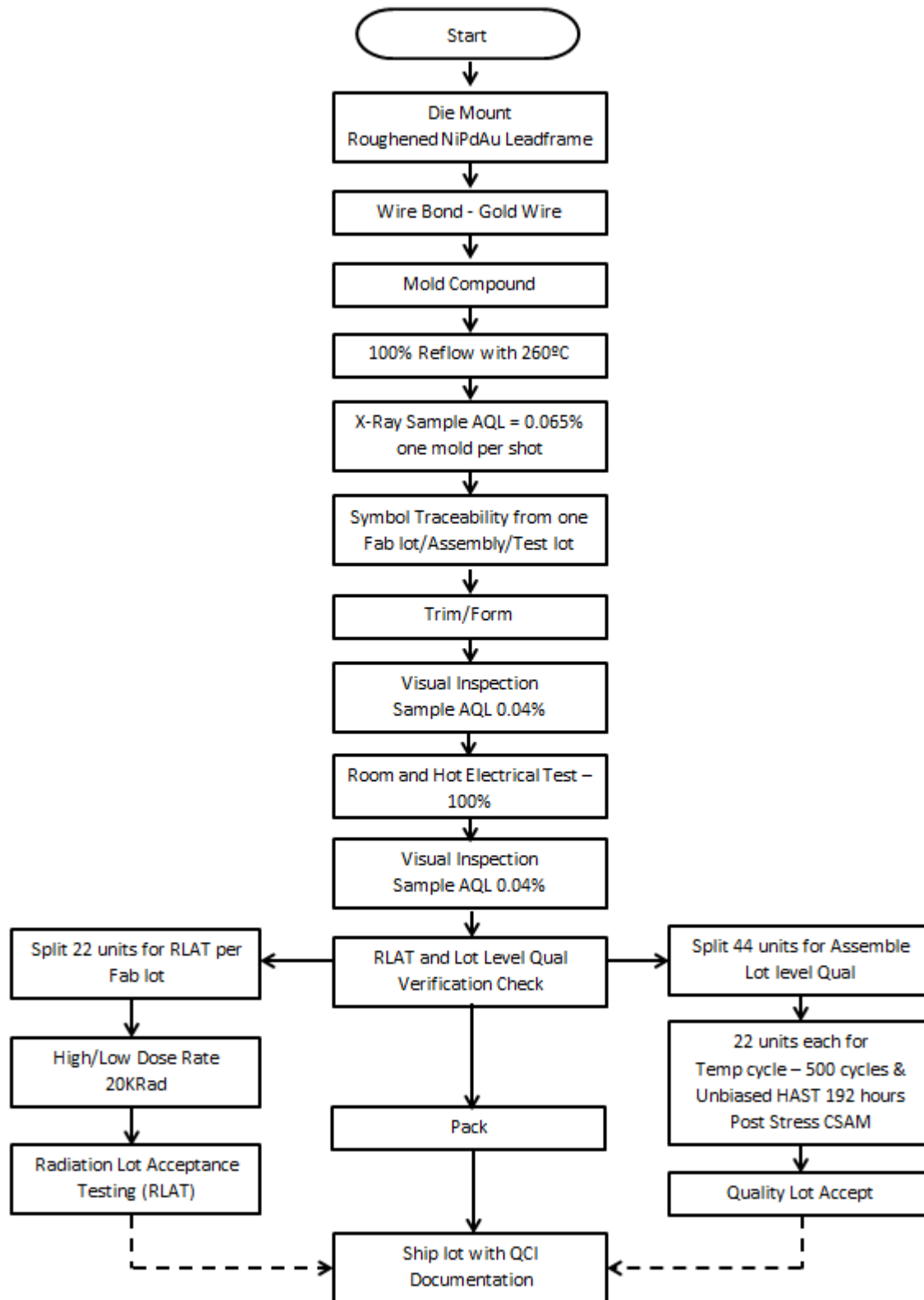
Figure 1. Space Enhanced Plastic Production Flow
