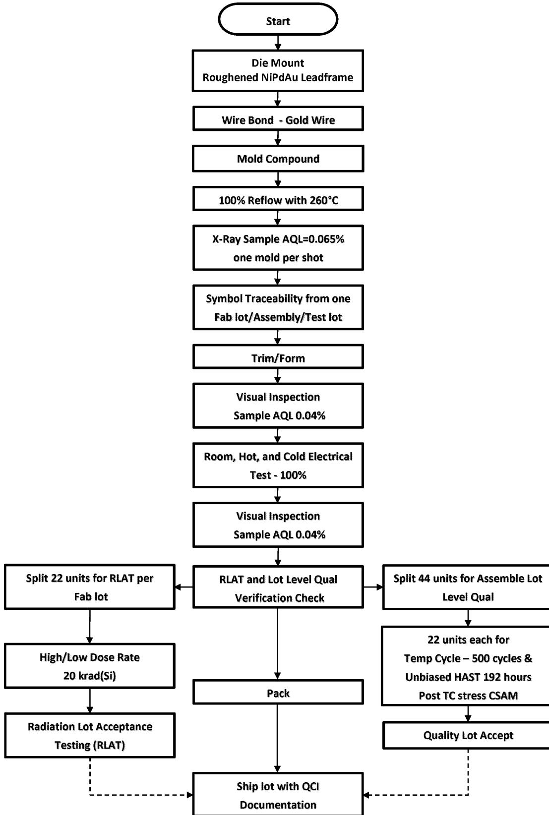
Figure 2-1. Space Enhanced Plastic Production Flow Chart
