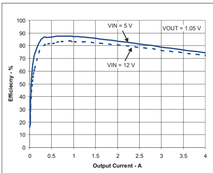
Figure 4-1. TPS54425EVM-608 Efficiency
