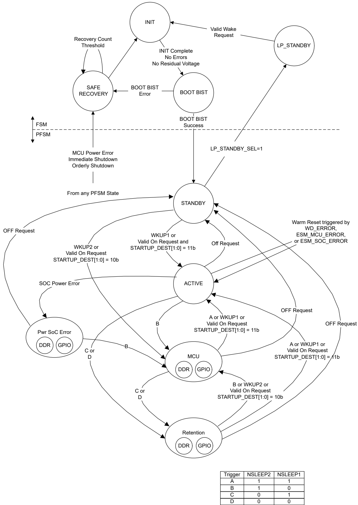
Figure 6-1. Pre-Configurable Finite State Machine (PFSM) Mission States and Transitions
