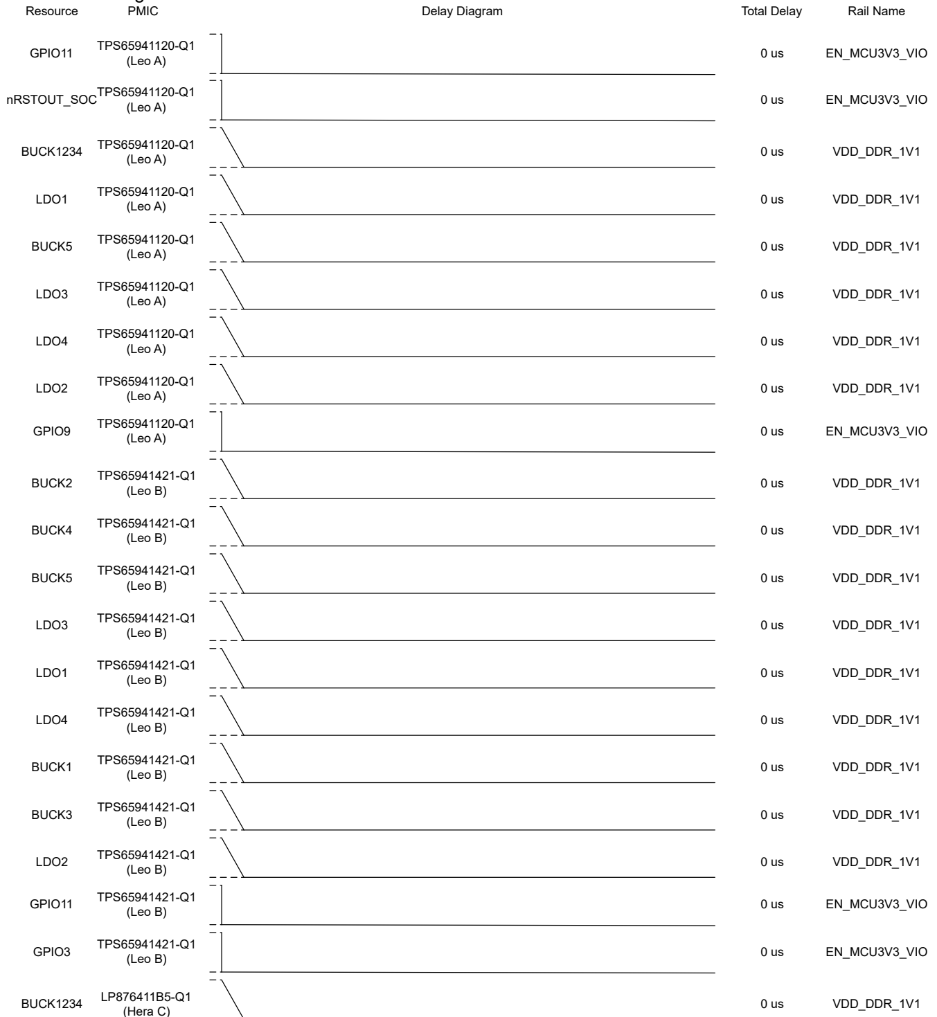
Figure 6-2. TO_SAFE_SEVERE and TO_SAFE Power Sequences
