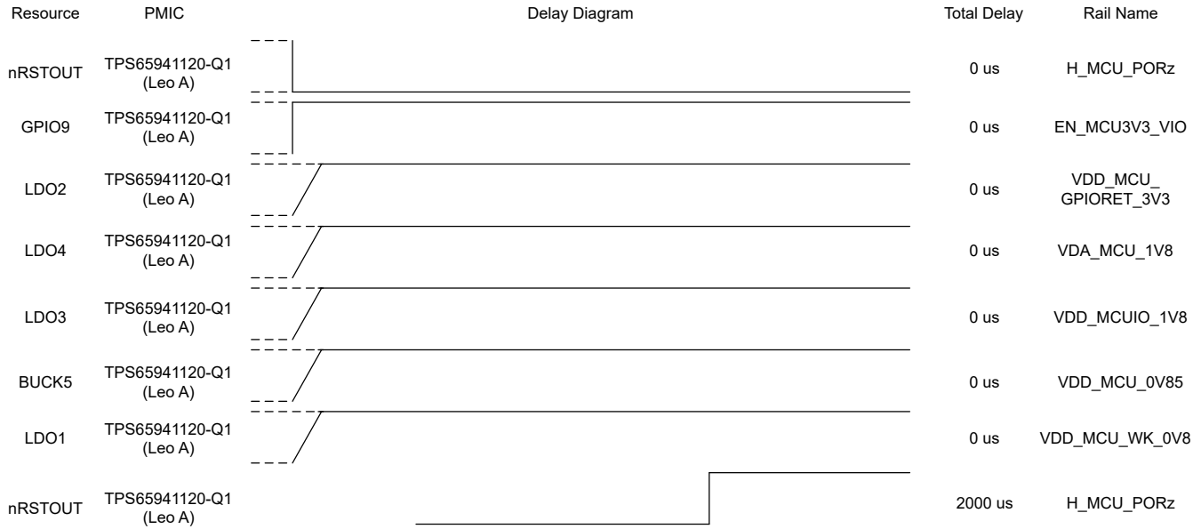
Figure 6-8. MCU_TO_WARM Sequence
