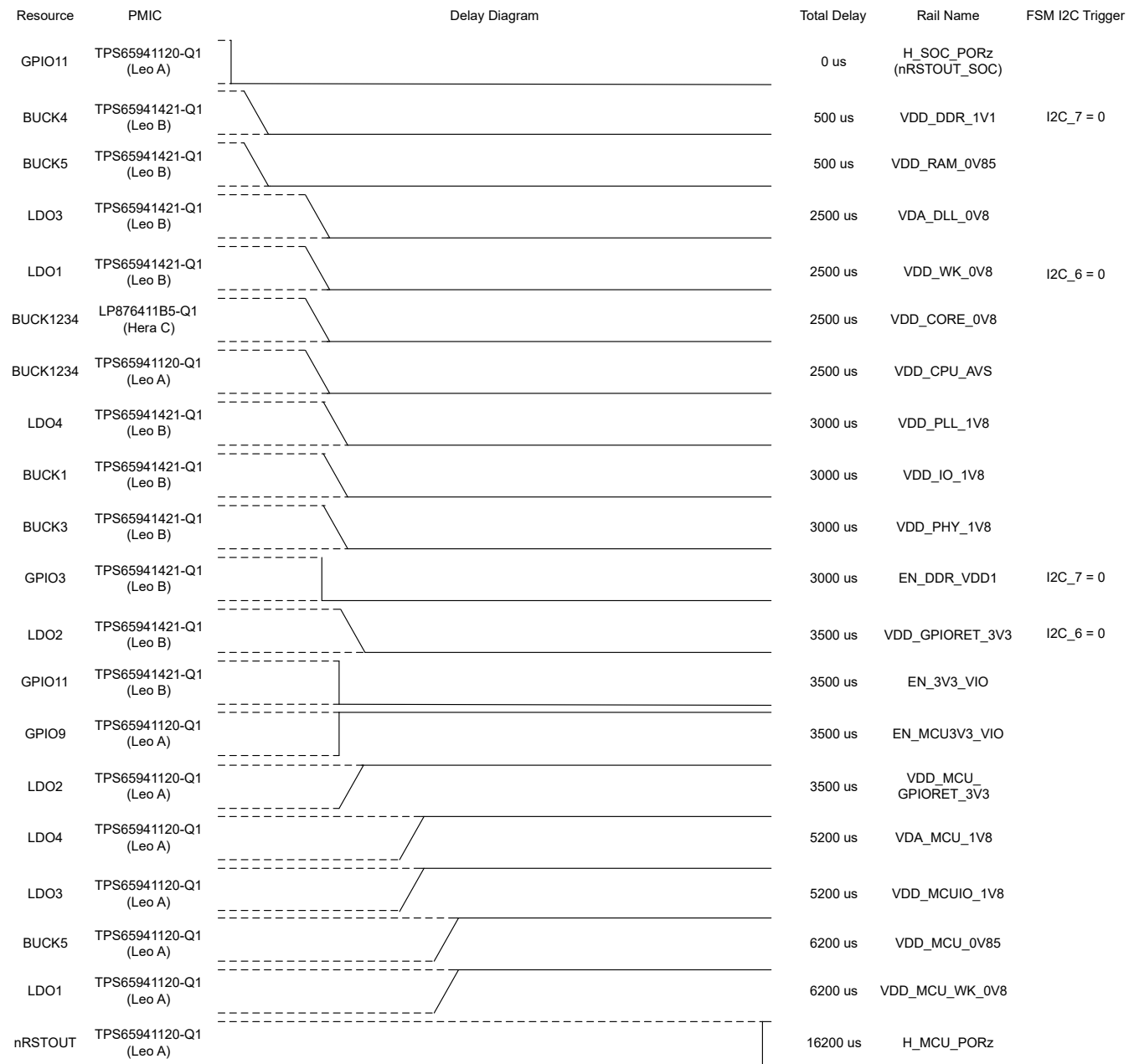
Figure 6-10. TO_MCU Sequence with I2C Triggers low in both PMICs
