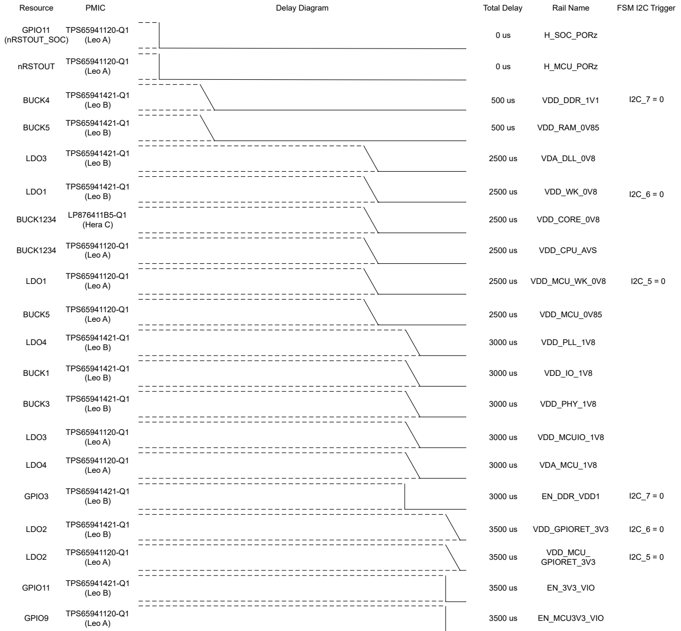
Figure 6-12. TO_RETENTION when I2C triggers are low in both PMICs
