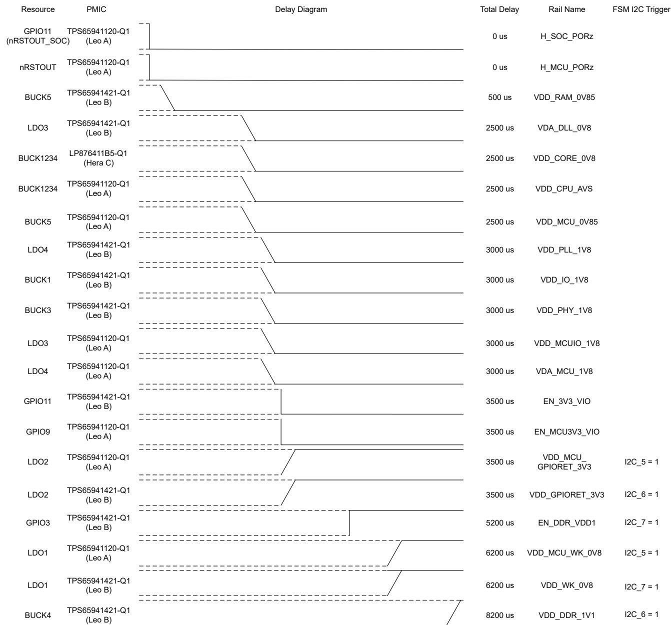
Figure 6-13. TO_RETENTION when I2C triggers are high in both PMICs
