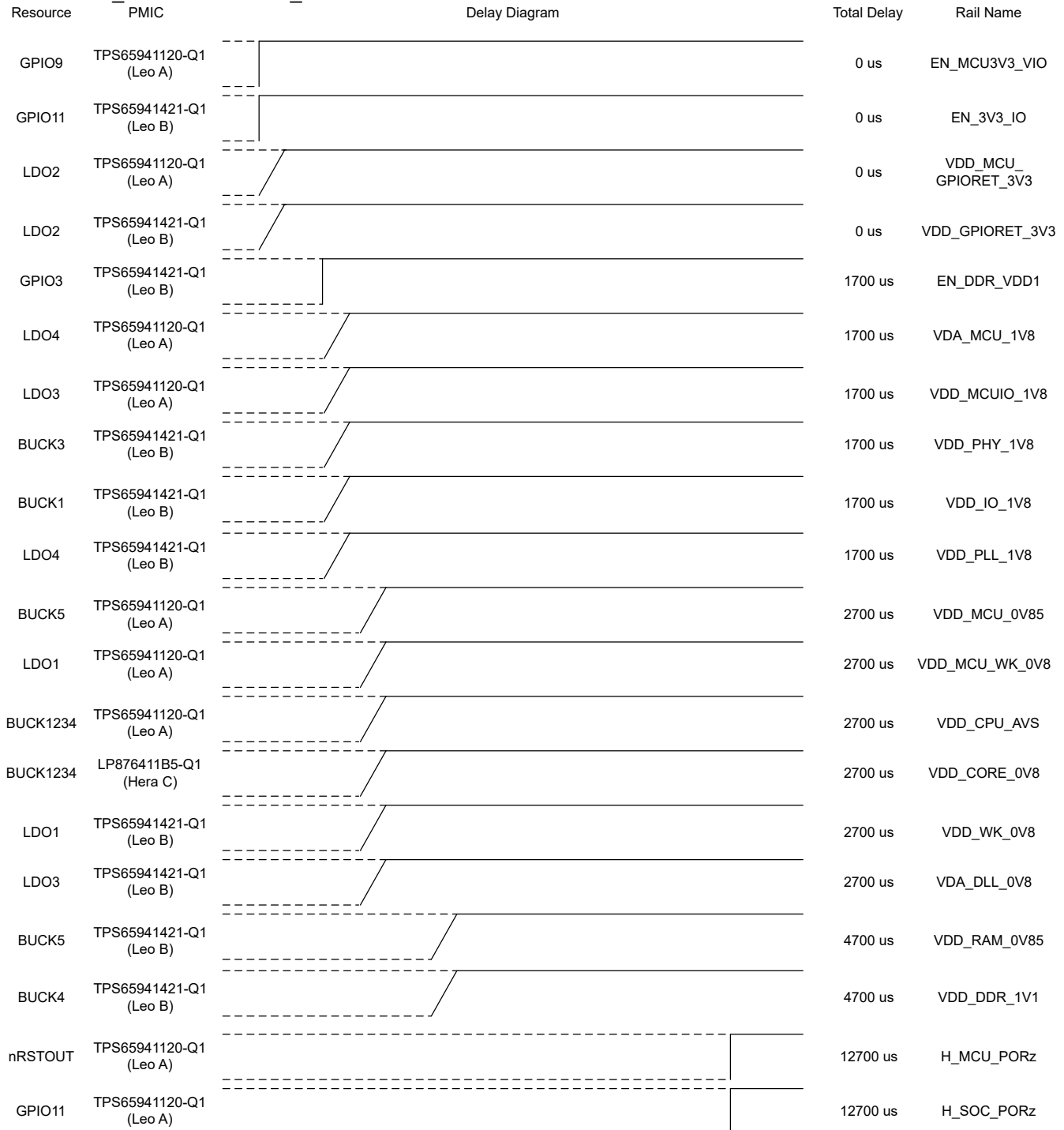
Figure 6-11. TO_ACTIVE Sequence
