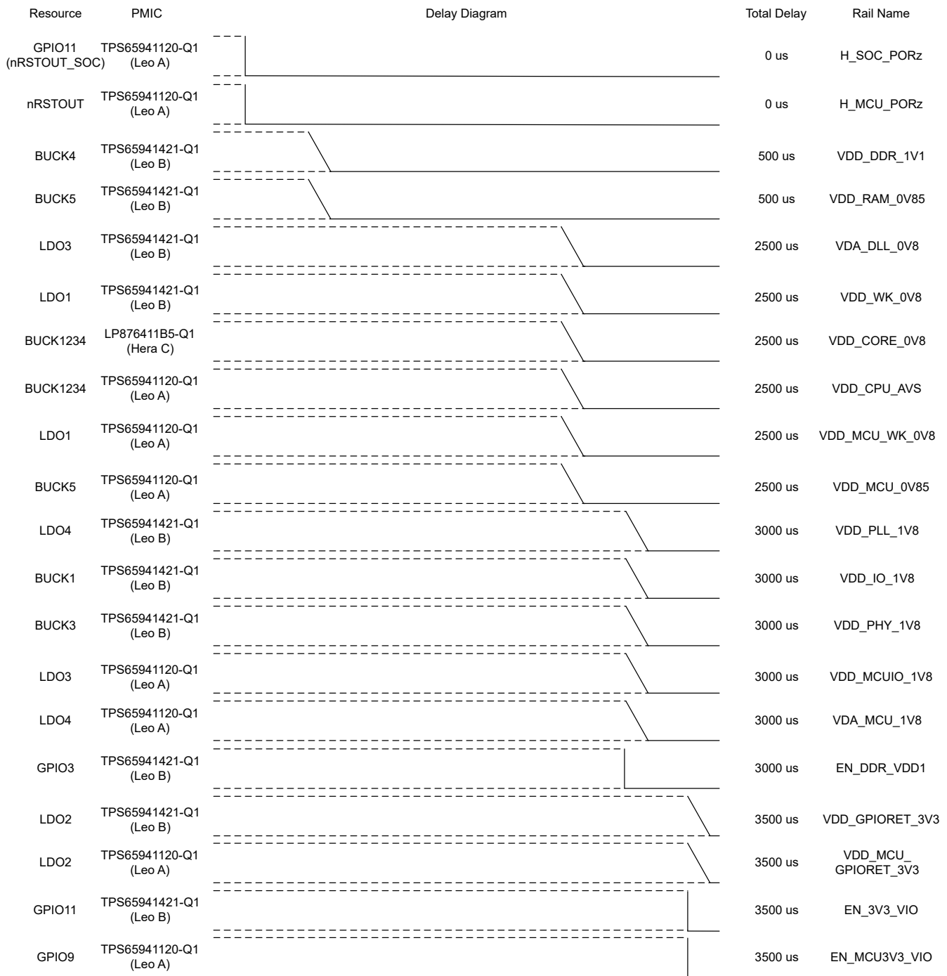
Figure 6-3. TO_SAFE_ORDERLY and TO_STANDBY Power Sequence
