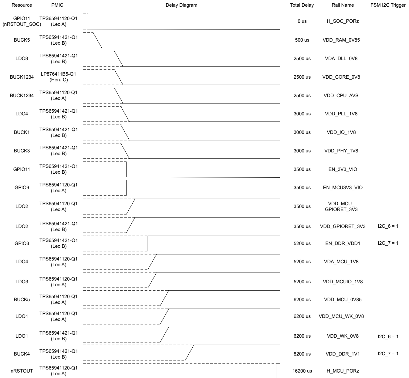
Figure 6-9. TO_MCU with I2C Triggers high in both PMICs
