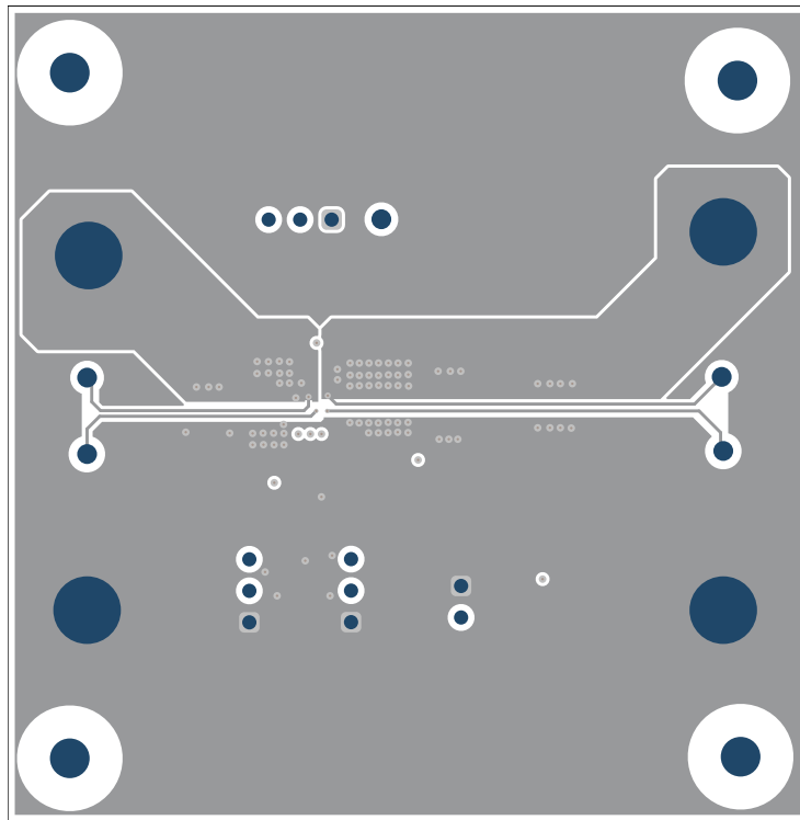
Figure 3-3. Bottom-Side Layout
