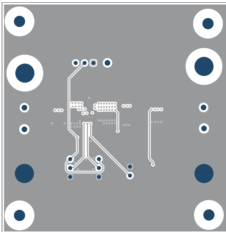
Figure 3-5. Inner Layer 2 Layout
