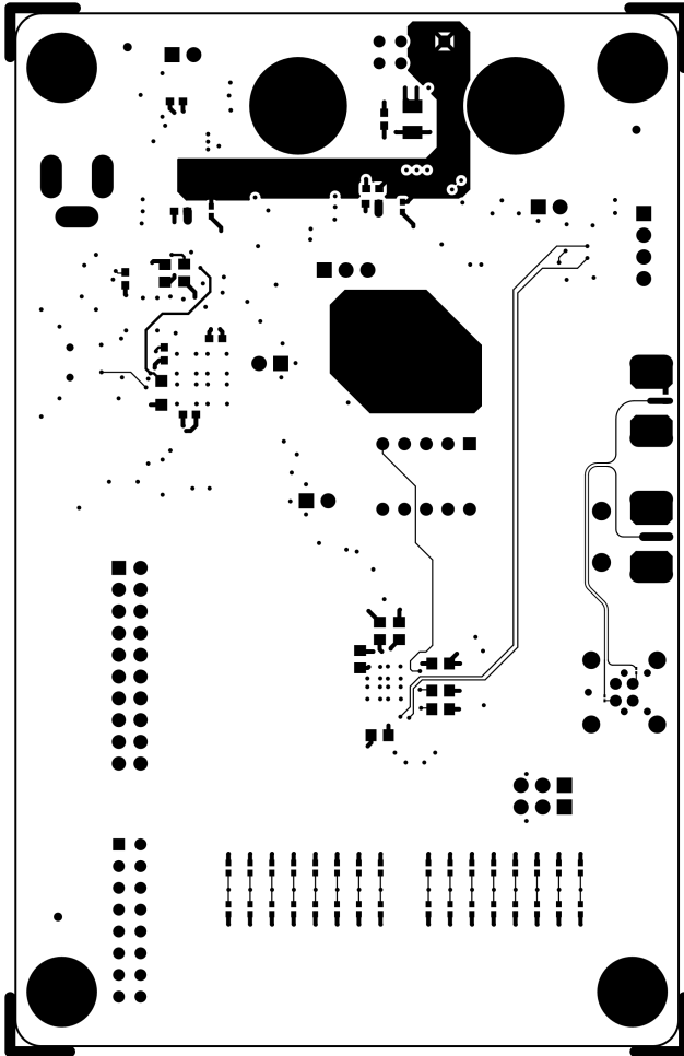
C-5. Bottom Copper
