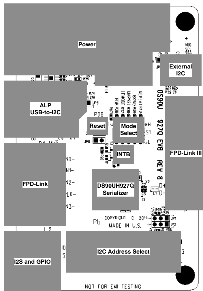
3-1. DS90UH927QEV M Layout
