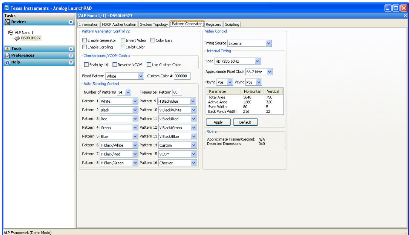
4-5. Pattern Generator Tab
