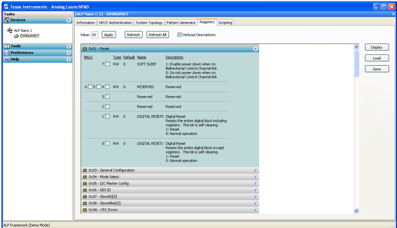
4-7. Register Tab with expanded register description
