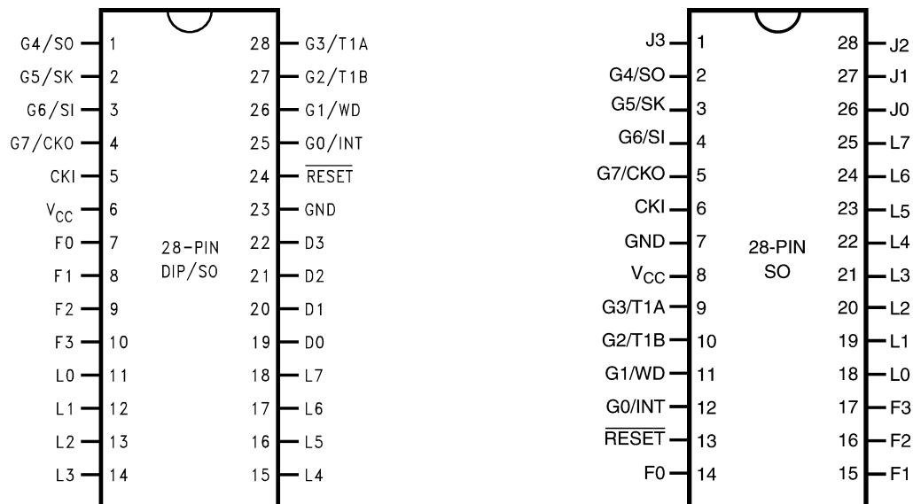
Figure 2. Comparative Pinouts for 28 Pin SOIC
