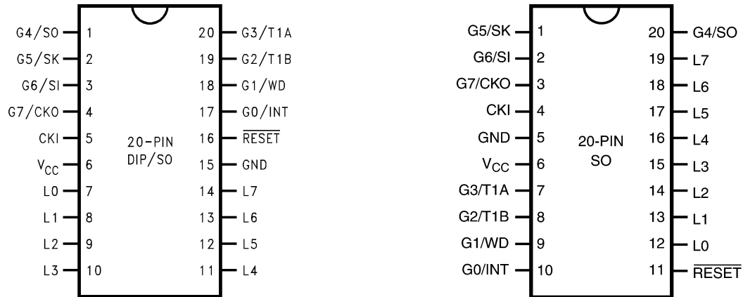
Figure 1. Comparative Pinouts for 20 Pin SOIC
