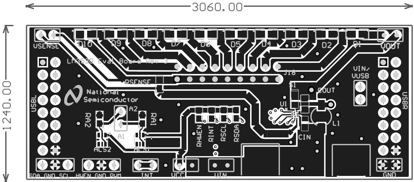
Figure 2. Top Layer
