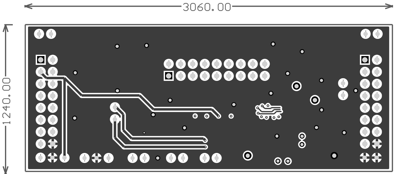
Figure 3. Mid Layer 1
