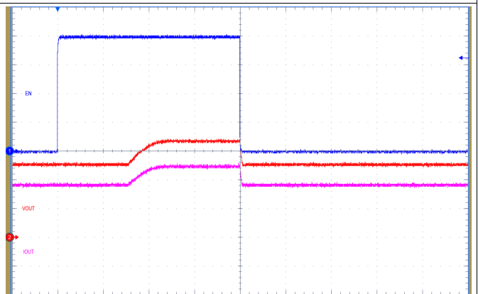
Figure 27. ENABLE On and Off with V_{OUT} Pre-biased to 3.3V; V_{IN} = 24\text{ V} , 500 mA Load (2ms/div, Ch1: V_{EN} , 1V/div; Ch2: V_{OUT} , 1V/div; Ch4: I_{OUT} , 200mA/div)
