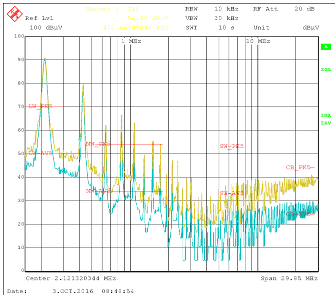
Figure 41. CISPR25 Class 5 Conducted Emissions Plot, 150 kHz to 30 MHz, VIN = 13.5 V, Load = 500 mA, UNFILTERED (Yellow: Peak Detector, Blue: Average Detector)
