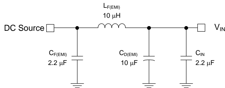
Figure 40. EMI Filter
