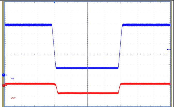
Figure 35. Line Transient Response, 500 mA Load 24 V to 3.5 V (Dropout) to 24 V at 0.1 V/ \mu s (1ms/div, Ch1: V IN , 10V/div; Ch2: V OUT , 500mV/div)
