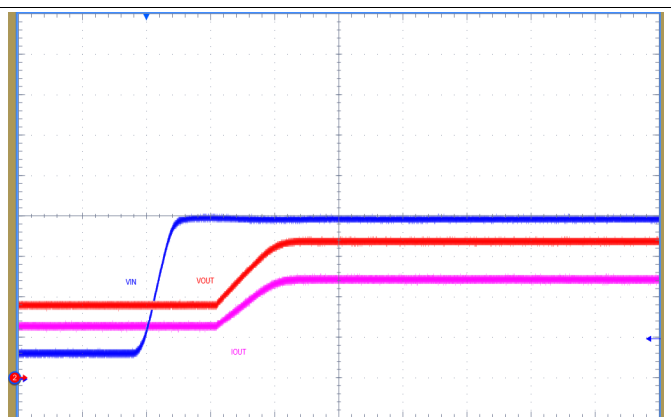
Figure 21. Startup with V_{OUT} Pre-biased to 1.8 V; V_{IN} = 12 V, 500 mA Load (2ms/div, Ch1: V_{IN} , 3V/div; Ch2: V_{OUT} , 1V/div; Ch4: I_{OUT} , 200mA/div)
