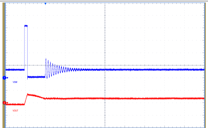
Figure 7. COT Mode SW Node and V_{OUT} Waveforms: V_{IN} = 24\text{ V} , V_{OUT} = 3.3\text{ V} , I_{OUT} = 0\text{ mA} (5 \mu\text{s}/\text{div} , Ch1: SW, 5V/div; Ch2: V_{OUT} , 50mV/div)
