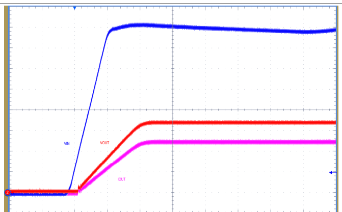
Figure 19. Startup with V_{IN} Ramping to 24 V, 500 mA Load (2ms/div, Ch1: V_{IN} , 3V/div; Ch2: V_{OUT} , 1V/div; Ch4: I_{OUT} , 200mA/div)
