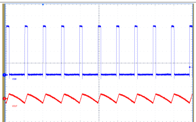
Figure 11. COT Mode SW Node and V_{OUT} Waveforms: V_{IN} = 24\text{ V} , V_{OUT} = 3.3\text{ V} , I_{OUT} = 500\text{ mA} (5 \mu\text{s}/\text{div} , Ch1: SW, 5V/div; Ch2: V_{OUT} , 50mV/div)
