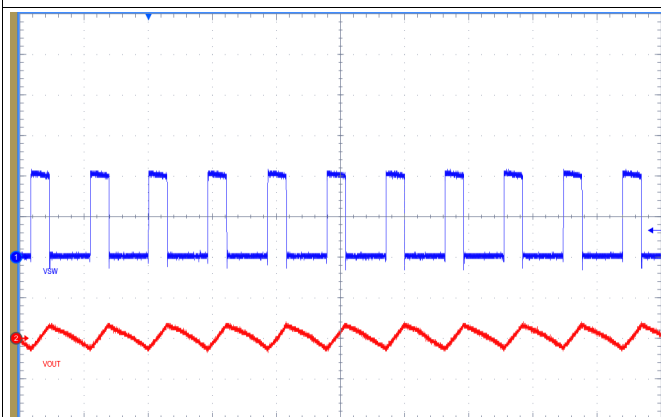
Figure 10. COT Mode SW Node and V_{OUT} Waveforms: V_{IN} = 12\text{ V} , V_{OUT} = 3.3\text{ V} , I_{OUT} = 500\text{ mA} (5 \mu\text{s}/\text{div} , Ch1: SW, 5V/div; Ch2: V_{OUT} , 50mV/div)
