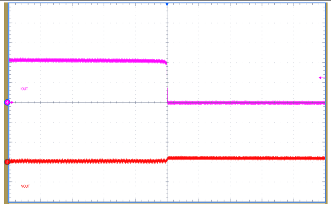
Figure 15. Load-OFF Transient Response V_{IN} = 24\text{ V} , V_{OUT} = 3.3\text{ V} , 500 mA to 0 mA at 2 A/ \mu s (100 \mu s/div, Ch4: I_{OUT} , 200mA/div; Ch2: V_{OUT} , 100mV/div)
