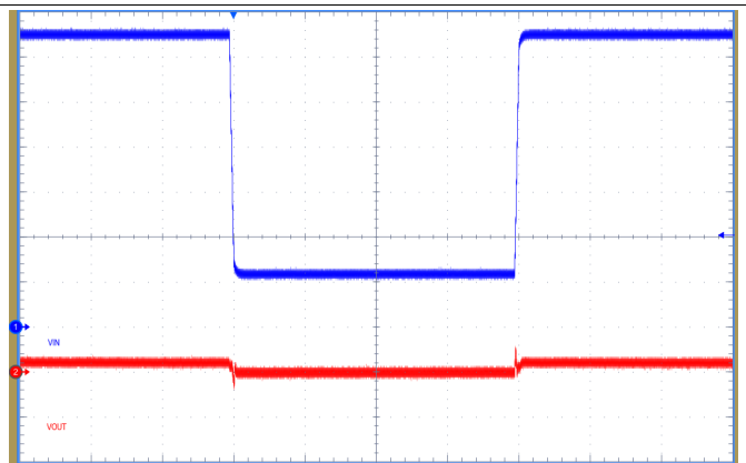
Figure 29. Line Transient Response, 500 mA Load 65 V to 12 V to 65 V at 1 V/μs (1ms/div, Ch1: V IN , 10V/div; Ch2: V OUT , 100mV/div)
