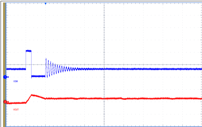
Figure 6. COT Mode SW Node and V_{OUT} Waveforms: V_{IN} = 12\text{ V} , V_{OUT} = 3.3\text{ V} , I_{OUT} = 0\text{ mA} (5 \mu\text{s}/\text{div} , Ch1: SW, 5V/div; Ch2: V_{OUT} , 50mV/div)
