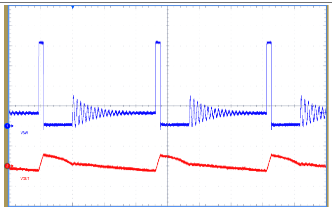
Figure 9. COT Mode SW Node and V_{OUT} Waveforms: V_{IN} = 24\text{ V} , V_{OUT} = 3.3\text{ V} , I_{OUT} = 50\text{ mA} (5 \mu\text{s}/\text{div} , Ch1: SW, 5V/div; Ch2: V_{OUT} , 50mV/div)
