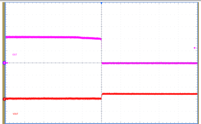
Figure 13. Load-OFF Transient Response V_{IN} = 12\text{ V} , V_{OUT} = 3.3\text{ V} , 500 mA to 0 mA at 2 A/ \mu s (100 \mu s/div, Ch4: I_{OUT} , 200mA/div; Ch2: V_{OUT} , 100mV/div)
