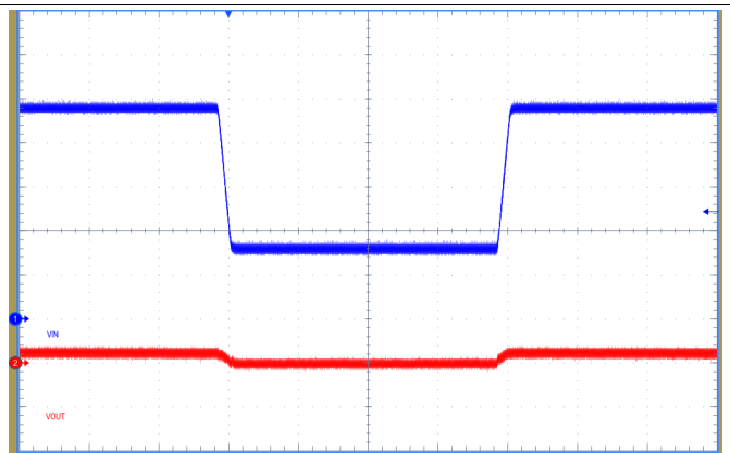
Figure 31. Line Transient Response, 500 mA Load 24 V to 8 V to 24 V at 0.1 V/μs (1ms/div, Ch1: V IN , 10V/div; Ch2: V OUT , 100mV/div)
