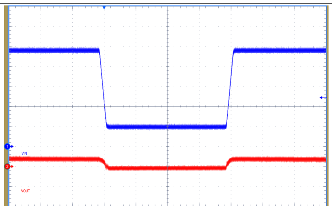
Figure 33. Line Transient Response, 500 mA Load 24 V to 5 V (Dropout) to 24 V at 0.1 V/μs (1ms/div, Ch1: V IN , 10V/div; Ch2: V OUT , 100mV/div)
