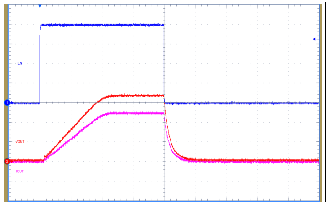
Figure 23. ENABLE On and Off; V_{IN} = 24\text{ V} , No Load (2ms/div, Ch1: V_{EN} , 1V/div; Ch2: V_{OUT} , 1V/div; Ch4: I_{OUT} , 200mA/div)
