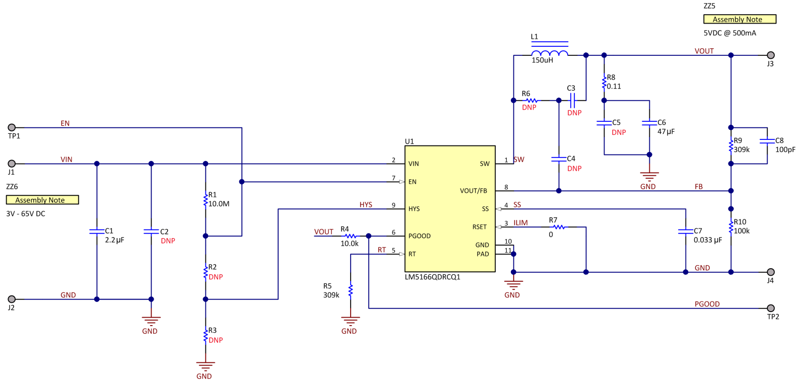
Figure 52. 5V, 500mA COT Schematic (Adjustable Output Version)
