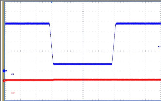
Figure 34. Line Transient Response, No Load 24 V to 3.5 V to 24 V at 0.1 V/ \mu s (1ms/div, Ch1: V IN , 10V/div; Ch2: V OUT , 100mV/div)
