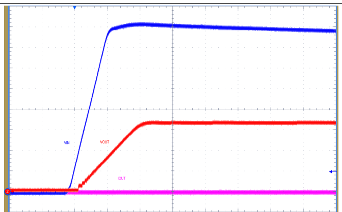
Figure 17. Startup with V_{IN} Ramping to 24 V, No Load (2ms/div, Ch1: V_{IN} , 3V/div; Ch2: V_{OUT} , 1V/div; Ch4: I_{OUT} , 200mA/div)
