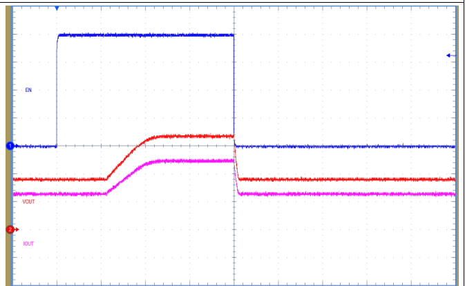
Figure 25. ENABLE On and Off with V_{OUT} Pre-biased to 1.8V; V_{IN} = 24\text{ V} , 500 mA Load (2ms/div, Ch1: V_{EN} , 1V/div; Ch2: V_{OUT} , 1V/div; Ch4: I_{OUT} , 200mA/div)
