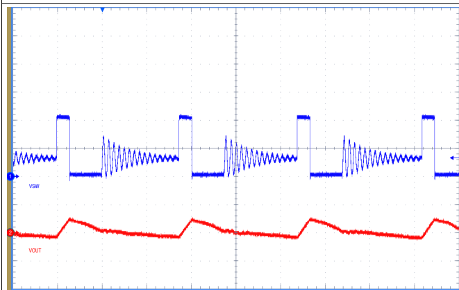
Figure 8. COT Mode SW Node and V_{OUT} Waveforms: V_{IN} = 12\text{ V} , V_{OUT} = 3.3\text{ V} , I_{OUT} = 50\text{ mA} (5 \mu\text{s}/\text{div} , Ch1: SW, 5V/div; Ch2: V_{OUT} , 50mV/div)
