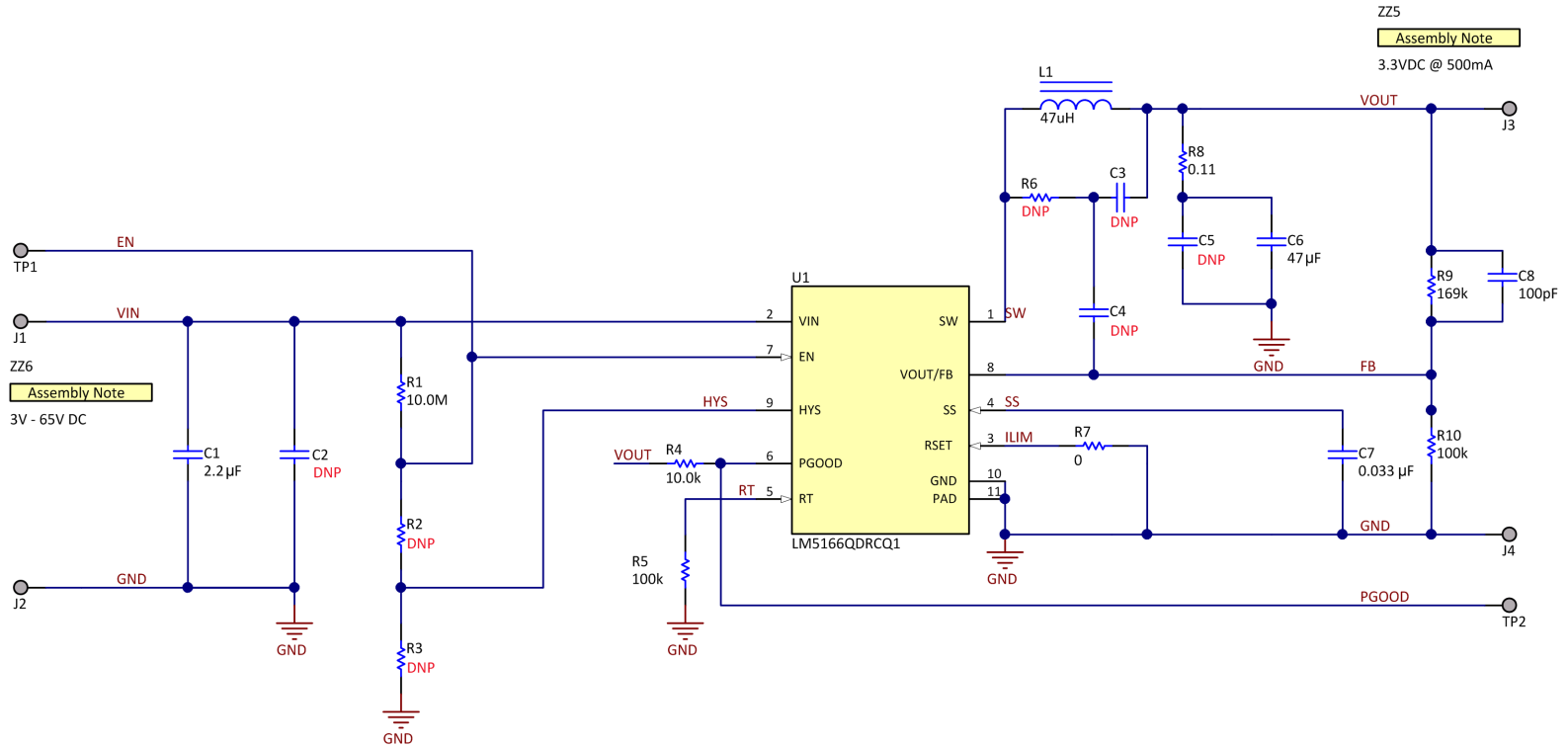
Figure 45. 3.3V, 500mA COT Schematic (Adjustable Output Version)
