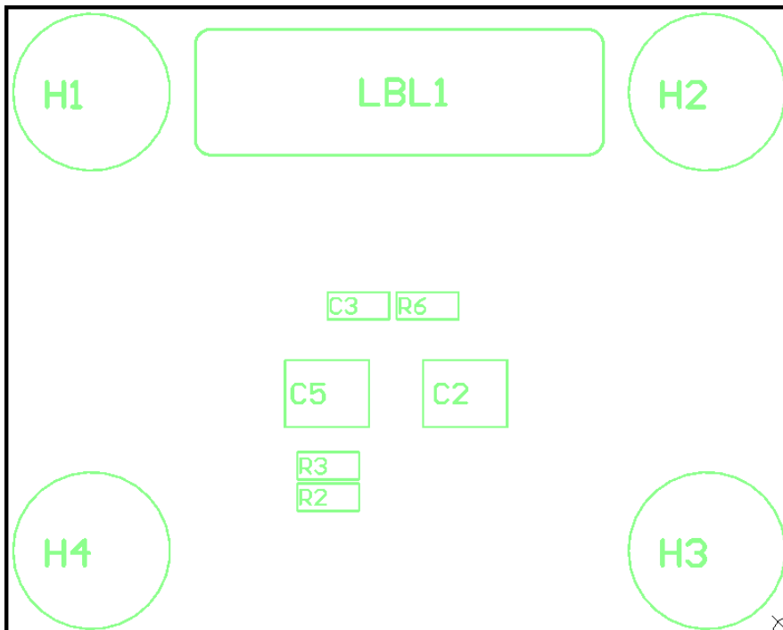
Figure 51. Bottom Assembly
