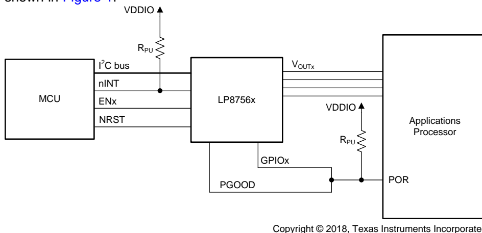
Figure 1. Typical MCU Connection to LP8756x-Q1 for Start-Up Configuration
