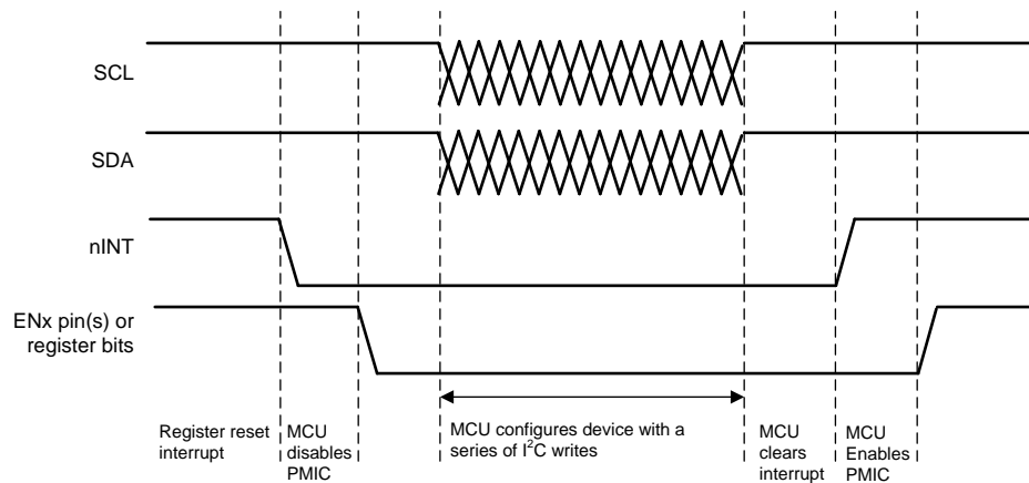
Figure 3. Configuration Sequence During Reset
