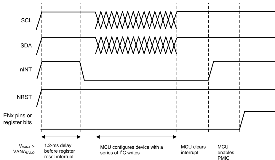
Figure 2. Configuration Sequence During Startup
