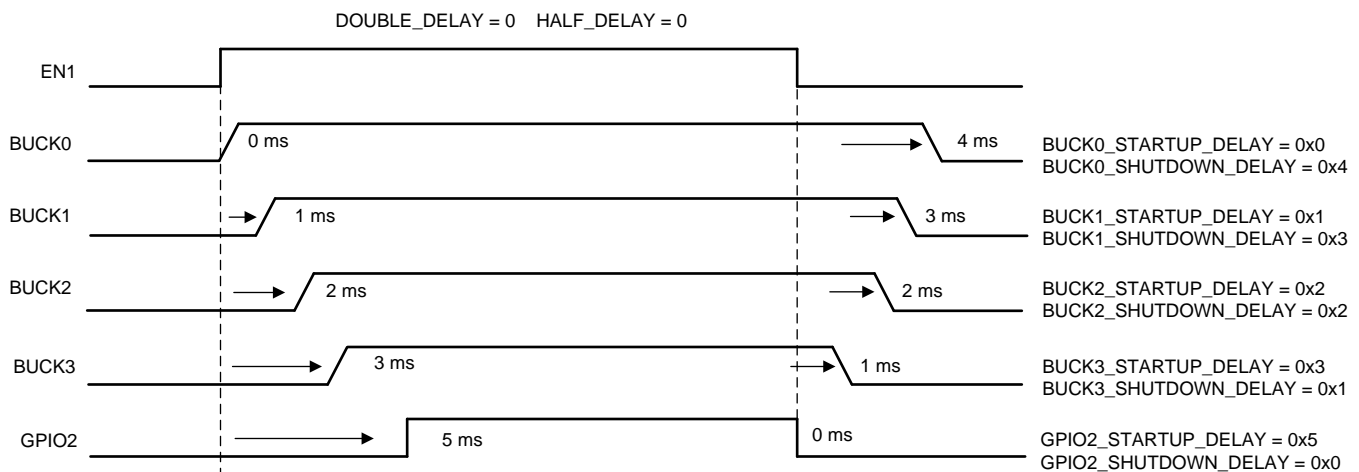
Figure 4. Startup and Shutdown Sequence Timing Diagram
