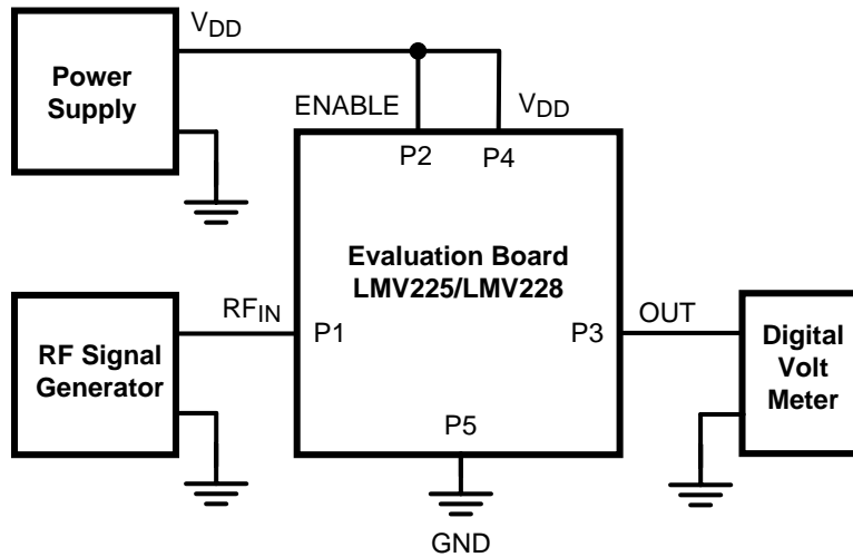
Figure 3. Measurement Setup
