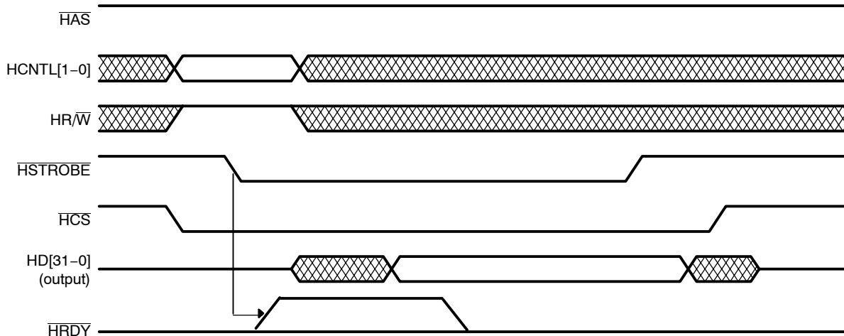
Figure 11. HPI32 Read Timing ( \overline{\text{HAS}} Not Used, Tied High) for C64x HPI
