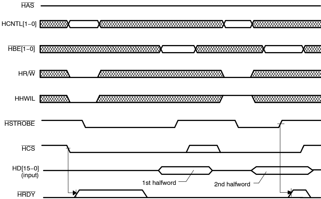
Figure 9. HPI Write Timing ( \overline{\text{HAS}} Not Used, Tied High)
