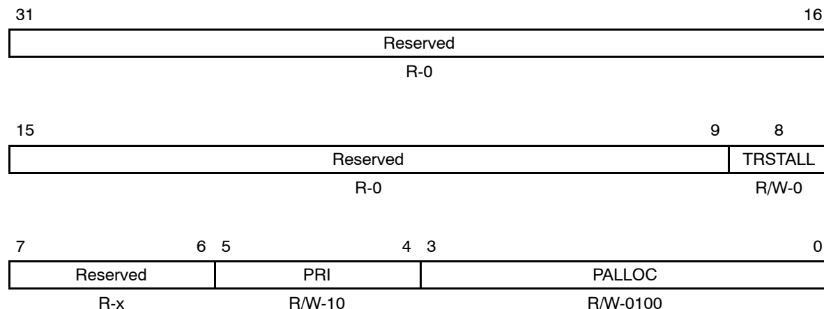
Figure 18. HPI Transfer Request Control Register (TRCTL)
