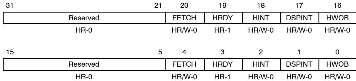
Figure 15. HPI Control Register (HPIC)—C620x/C670x DSP
