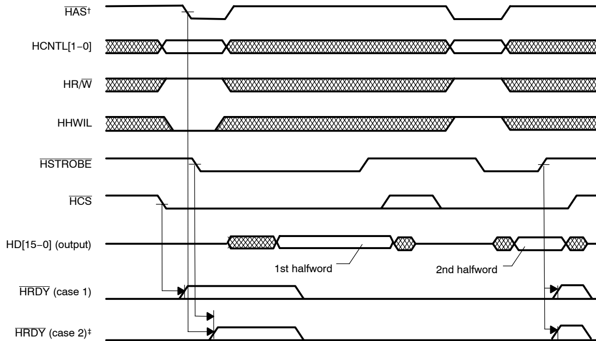
Figure 8. HPI Read Timing ( \overline{\text{HAS}} Used)
