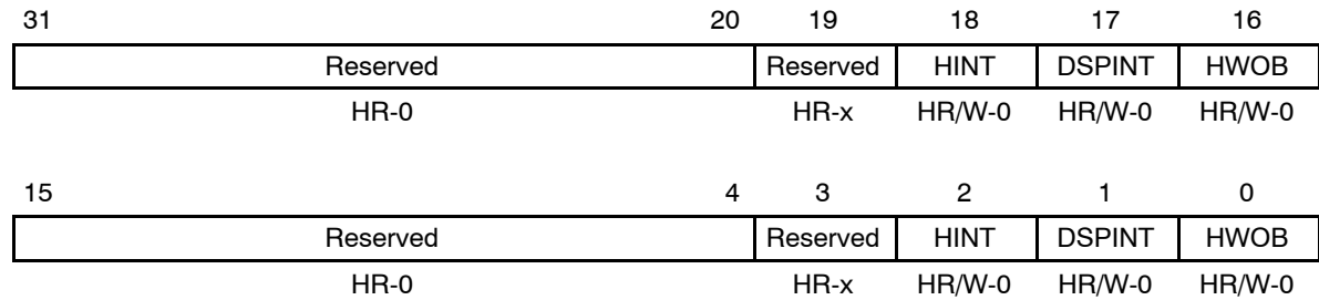
Figure 16. HPI Control Register (HPIC)—C621x/C671x DSP
