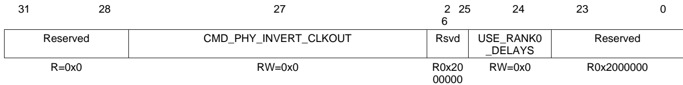
Figure 4-42. DDR3 Configuration 12 Register (DDR3_CONFIG_12)
