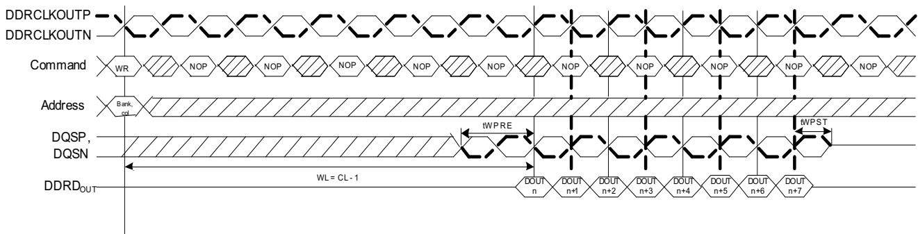
Figure 2-3. WRITE Command
