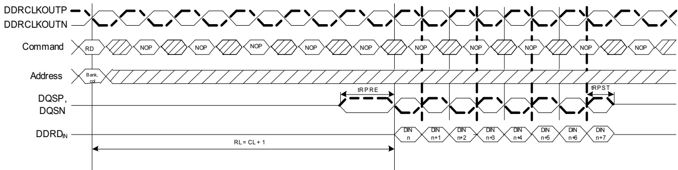
Figure 2-2. READ Command
