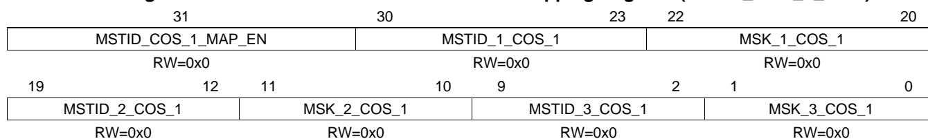
Figure 4-25. Master ID to Class-Of-Service 1 Mapping Register (MSTID_COS_1_MAP)
