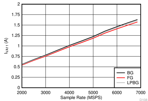
Figure 5-124. DES Mode: I_{VA11} vs Sample Rate
