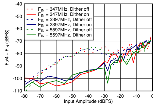
Figure 5-70. DES Mode: F_{\text{s}/4} + F_{\text{IN}} vs Input Amplitude and Dither
