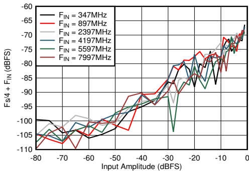
Figure 5-69. DES Mode: F_{\text{s}/4} + F_{\text{IN}} vs Input Amplitude and Frequency
