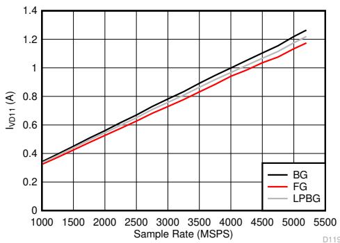
Figure 5-135. Dual Channel Mode: I_{VD11} vs Sample Rate
