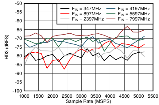
Figure 5-56. Dual Channel Mode: HD3 vs Sample Rate and Input Frequency
