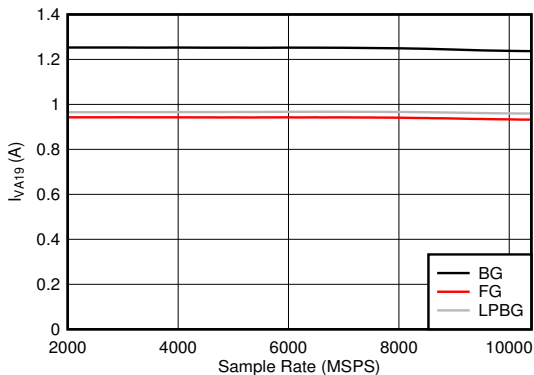
Figure 5-123. DES Mode: I_{VA19} vs Sample Rate
