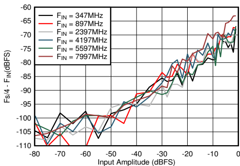
Figure 5-71. DES Mode: F_{\text{s}/4} - F_{\text{IN}} vs Input Amplitude and Frequency
