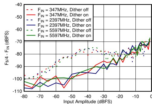
Figure 5-72. DES Mode: F_{\text{s}/4} - F_{\text{IN}} vs Input Amplitude and Dither
