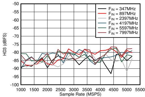
Figure 5-55. Dual Channel Mode: HD3 vs Sample Rate and Input Frequency
