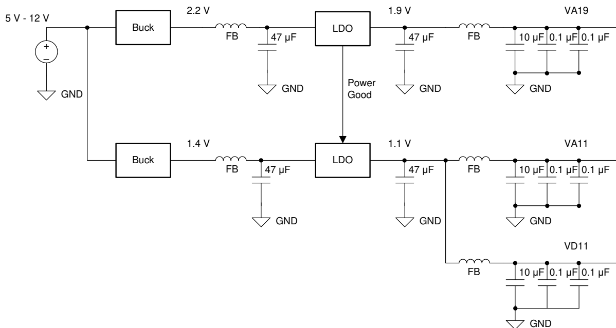
Figure 7-5. LDO Linear Regulator Approach Example
