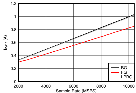
Figure 5-124. DES Mode: I_{VA11} vs Sample Rate
