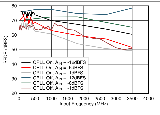
Figure 7-48. SFDR vs A_{IN} and C-PLL
