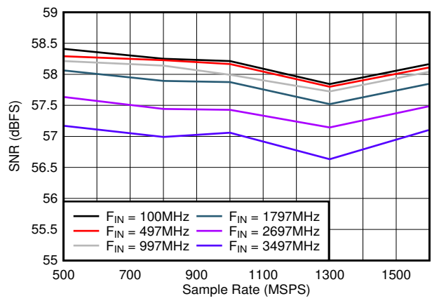
Figure 7-24. SNR vs Sample Rate
