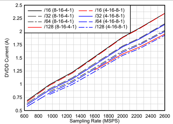
A_{IN} = -1\text{ dBFS} , 1x AVG, Dither = DIS Quad Band Decimation
