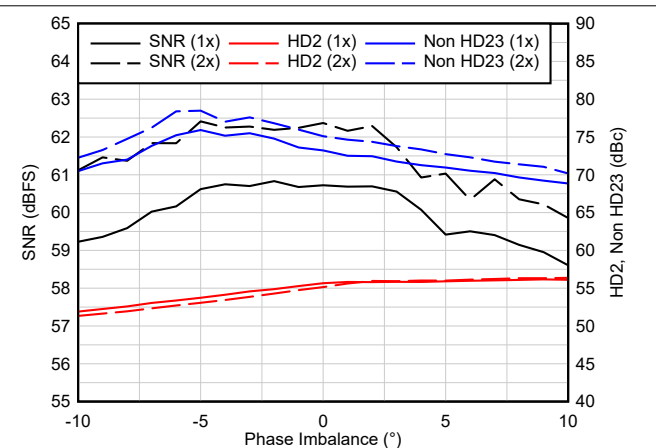
Figure 7-6. Phase Imbalance - 3.0 GSPS
