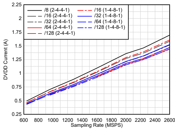
A_{IN} = -1\text{ dBFS} , 1x AVG, Dither = DIS Single Band Decimation
