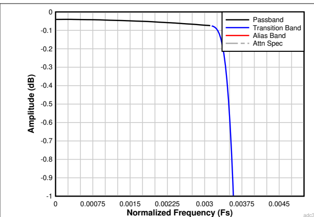
Figure 7-37. Decimation by 128 Passband Ripple Response
