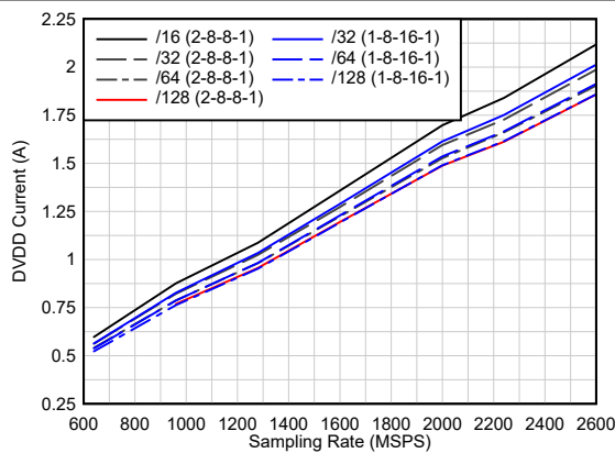
A_{IN} = -1\text{ dBFS} , 1x AVG, Dither = DIS Dual Band Decimation
