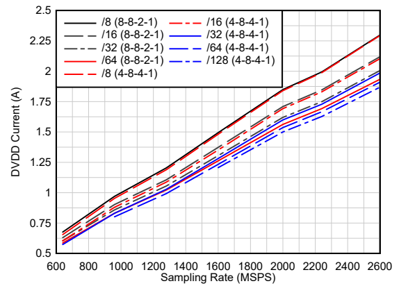
A_{IN} = -1\text{ dBFS} , 1x AVG, Dither = DIS Dual Band Decimation
