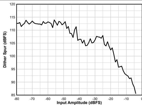
F_{IN} = 900 MHz, Figure 6-84. Dither Spur vs A_{IN}
