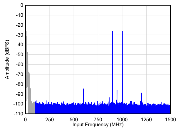
IMD3 = 71 dBc A_{IN} = -26 dBFS/tone, 1x AVG, Dither = EN
