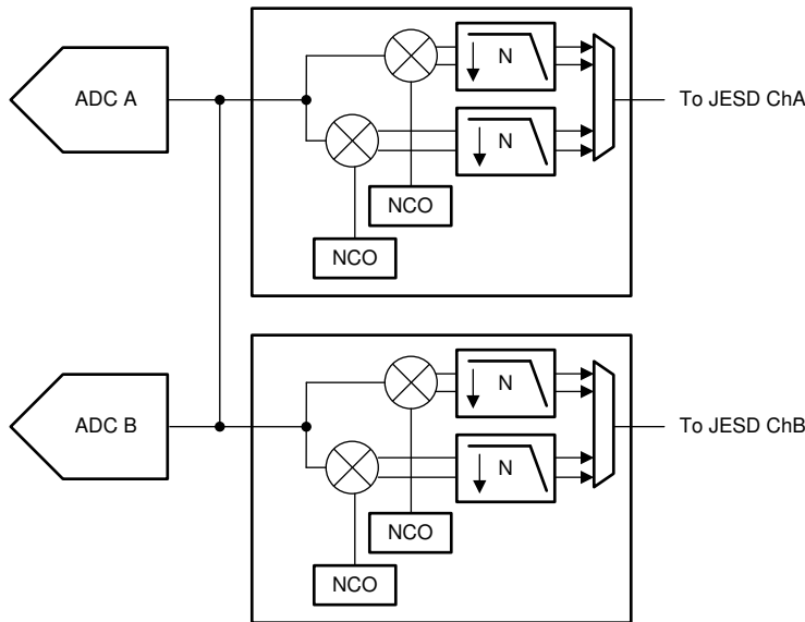
Figure 8-41. Digital Multiplexer Option
