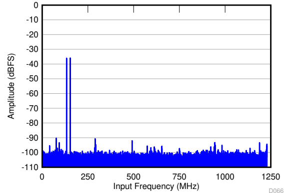
f_{IN1} = 2.59 \text{ GHz} , f_{IN2} = 2.6 \text{ GHz} , A_{IN} = -36 \text{ dBFS} , \text{IMD} = 92 \text{ dBFS}
