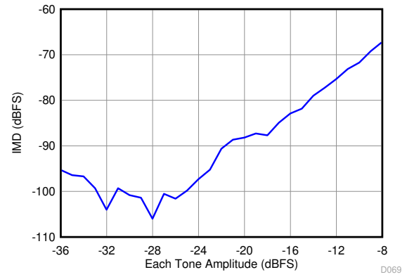
Figure 6-36. Intermodulation Distortion vs. Input Amplitude (3490 MHz and 3510 MHz, f_s = 2457.6 \text{ MSPS} )
