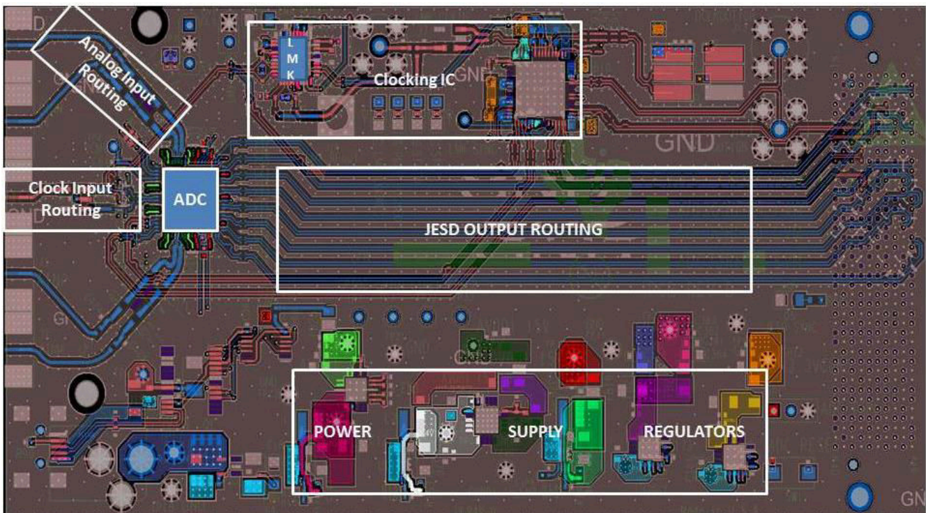
Figure 11-1. ADC32RF8xEVM Layout
