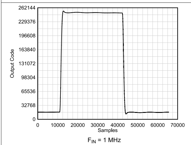
Figure 6-62. Pulse Response
