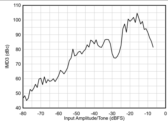
Figure 6-15. AC Performance vs A_{IN} F_{IN} = 100\text{MHz}
