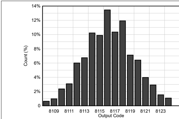
Figure 6-25. DC Offset Histogram
