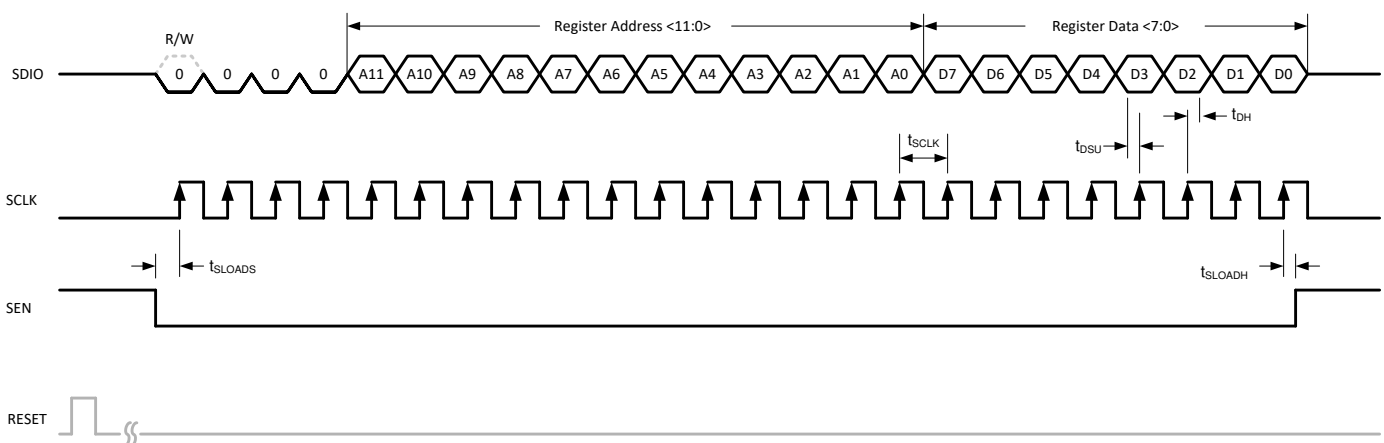
Figure 8-75. Serial Register Write Timing Diagram
