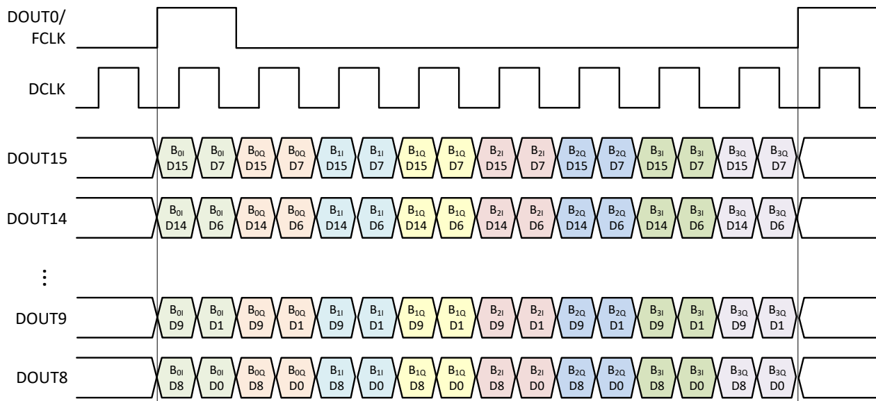
Figure 8-59. SLVDS frame assembly for example 4
