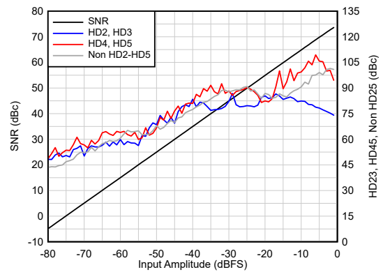
Figure 6-14. AC Performance vs A_{IN} F_{IN} = 10\text{MHz}
