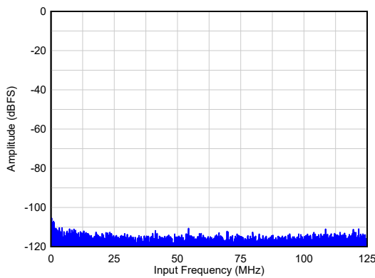
Figure 6-27. Idle Channel Noise
