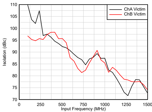
Figure 6-45. Isolation vs F_{IN}
