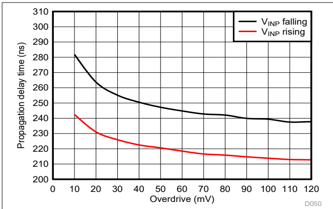
Figure 5-54. Cmp1 Propagation Delay vs Overdrive
