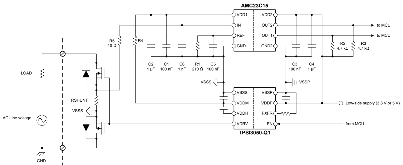
Figure 7-1. Using the AMC23C15 for Overcurrent and Short-Circuit Detection
