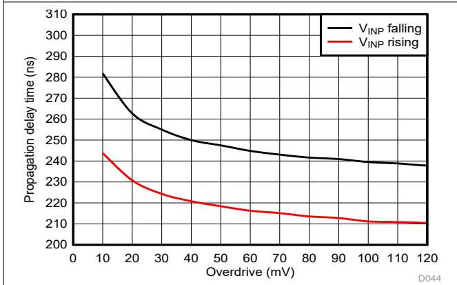
Figure 5-48. Cmp2 Propagation Delay vs Overdrive
