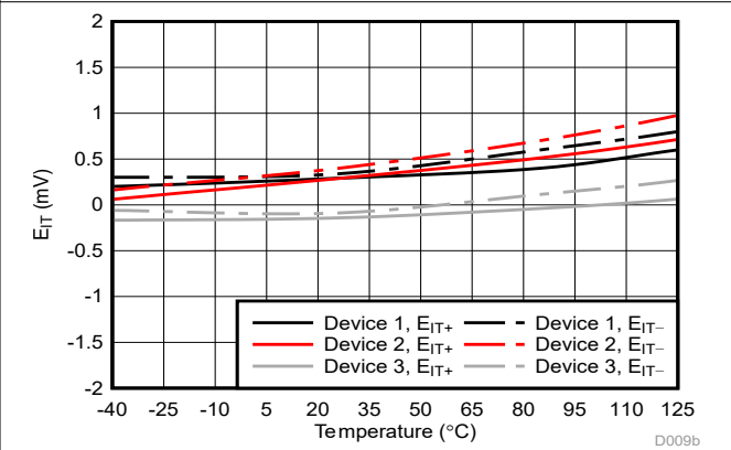
Figure 5-7. Cmp2 Trip Threshold vs Temperature
