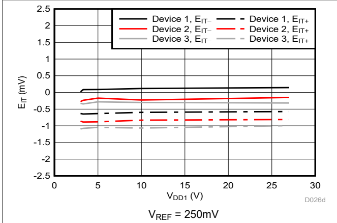
Figure 5-44. Cmp1 Trip Threshold Error vs Supply Voltage
