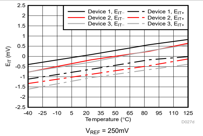
Figure 5-45. Cmp1 Trip Threshold Error vs Temperature
