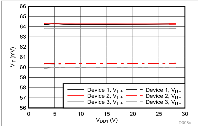
Figure 5-6. Cmp2 Trip Threshold vs Supply Voltage
