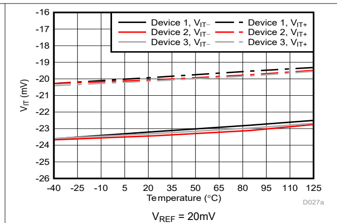
Figure 5-37. Cmp1 Trip Threshold vs Temperature
