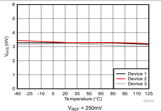
Figure 5-47. Cmp1 Trip Threshold Hysteresis vs Temperature
