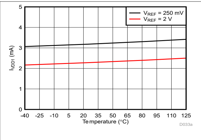
Figure 5-61. High-Side Supply Current vs Temperature
