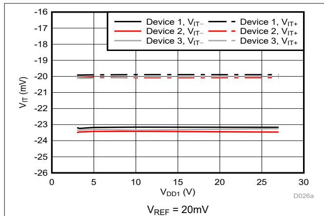
Figure 5-36. Cmp1 Trip Threshold vs Supply Voltage
