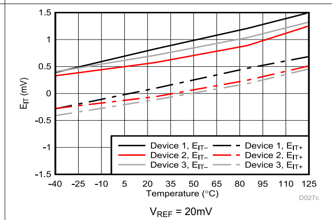
Figure 5-39. Cmp1 Trip Threshold Error vs Temperature
