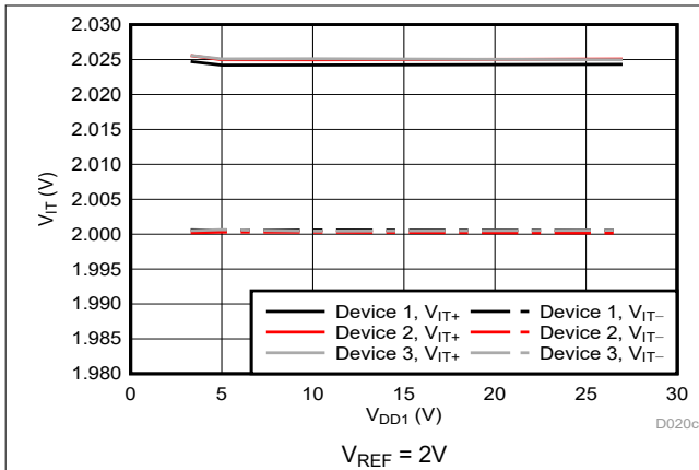
Figure 5-30. Cmp0 Trip Threshold vs Supply Voltage
