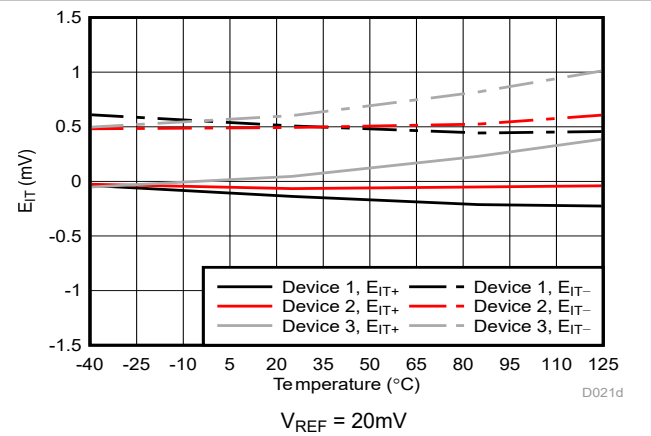
Figure 5-21. Cmp0 Trip Threshold Error vs Temperature
