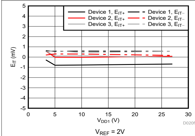
Figure 5-32. Cmp0 Trip Threshold Error vs Supply Voltage
