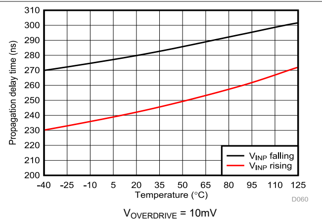
Figure 5-51. Cmp3 Propagation Delay vs Temperature
