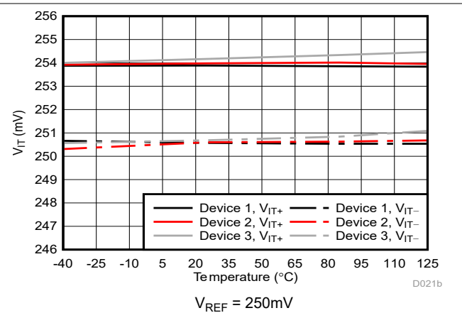
Figure 5-25. Cmp0 Trip Threshold vs Temperature
