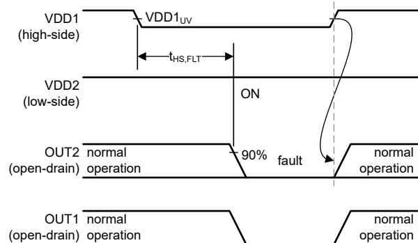
Figure 6-12. Output Response to a Long Brownout Event on VDD1
