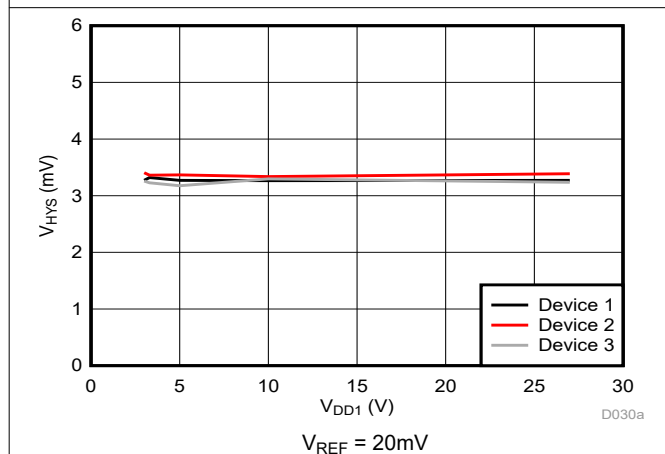
Figure 5-40. Cmp1 Trip Threshold Hysteresis vs Supply Voltage
