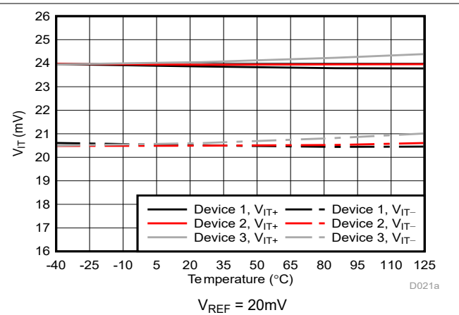
Figure 5-19. Cmp0 Trip Threshold vs Temperature
