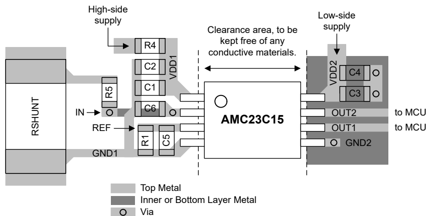
Figure 7-8. Recommended Layout of the AMC23C15
