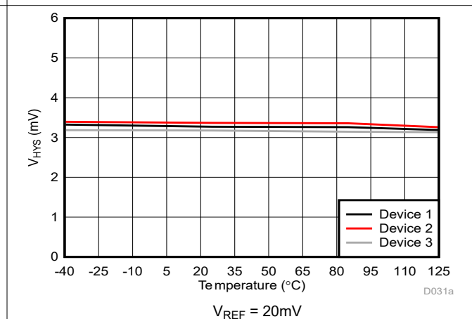
Figure 5-41. Cmp1 Trip Threshold Hysteresis vs Temperature
