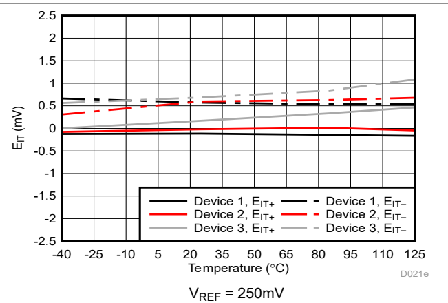
Figure 5-27. Cmp0 Trip Threshold Error vs Temperature
