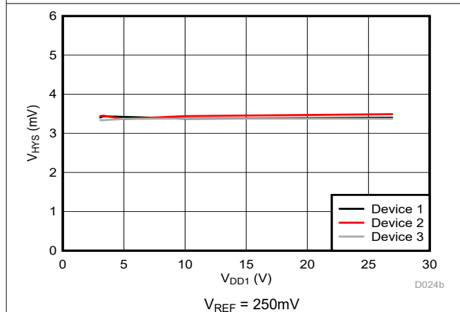
Figure 5-28. Cmp0 Trip Threshold Hysteresis vs Supply Voltage
