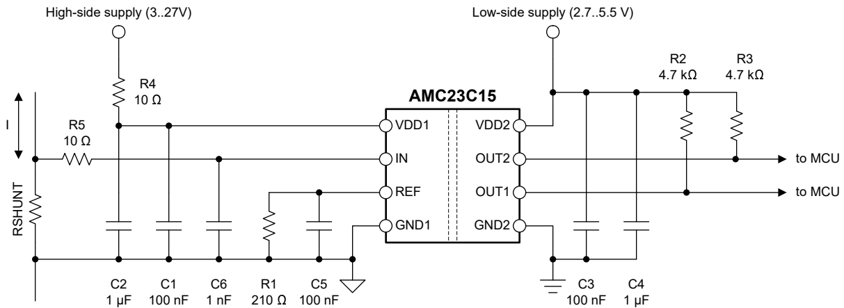
Figure 7-7. Decoupling of the AMC23C15
