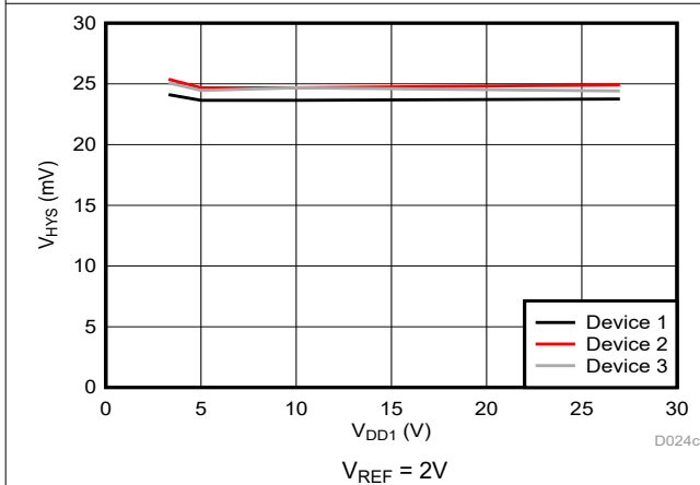
Figure 5-34. Cmp0 Trip Threshold Hysteresis vs Supply Voltage
