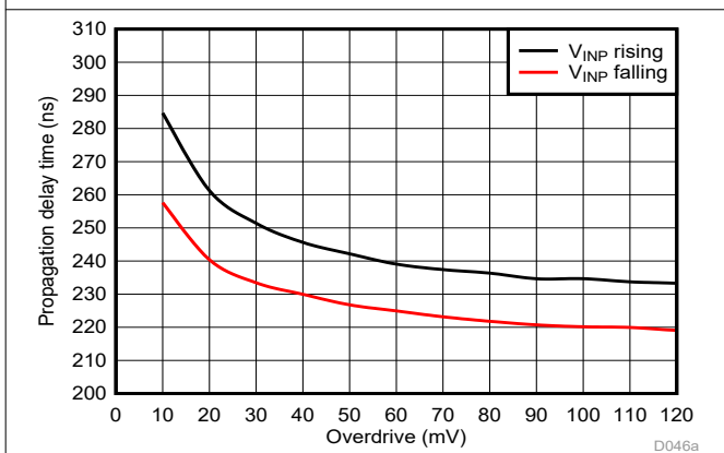
Figure 5-50. Cmp3 Propagation Delay vs Overdrive
