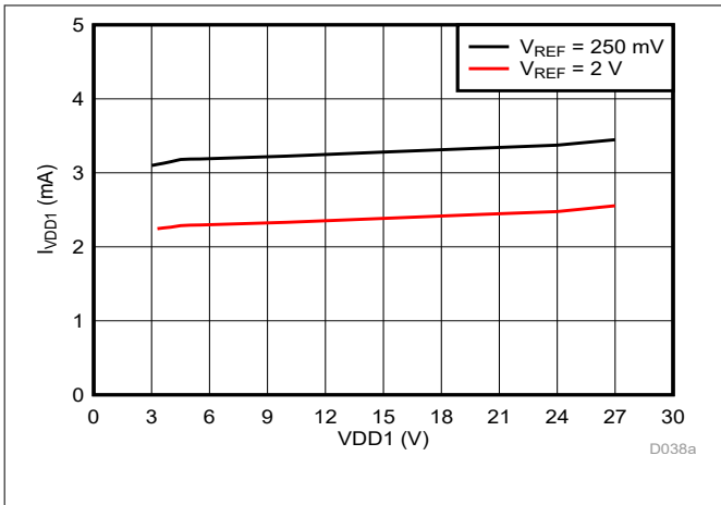
Figure 5-60. High-Side Supply Current vs Supply Voltage
