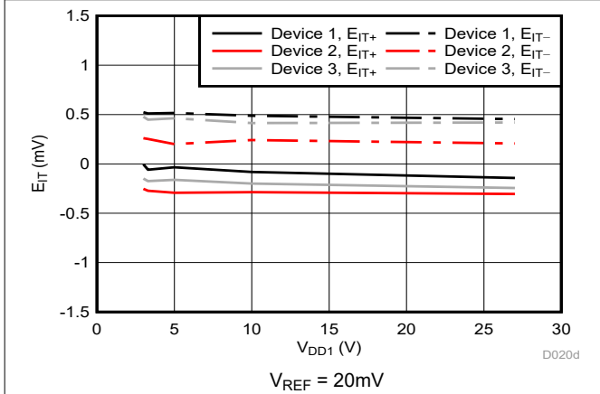
Figure 5-20. Cmp0 Trip Threshold Error vs Supply Voltage
