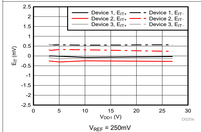
Figure 5-26. Cmp0 Trip Threshold Error vs Supply Voltage
