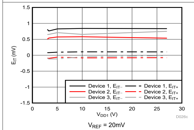
Figure 5-38. Cmp1 Trip Threshold Error vs Supply Voltage
