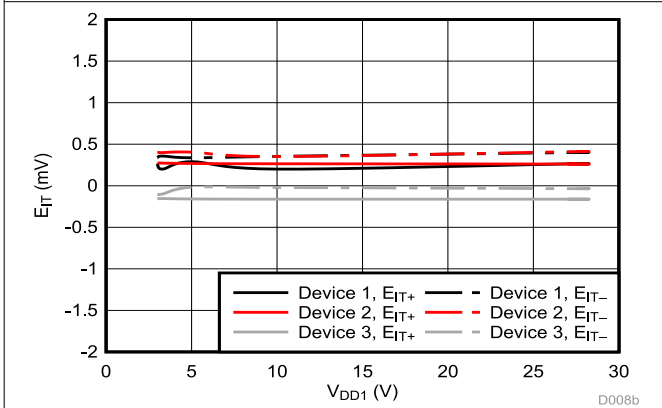
Figure 5-6. Cmp2 Trip Threshold vs Supply Voltage
