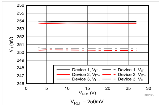
Figure 5-24. Cmp0 Trip Threshold vs Supply Voltage
