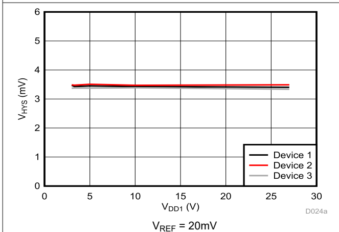
Figure 5-22. Cmp0 Trip Threshold Hysteresis vs Supply Voltage
