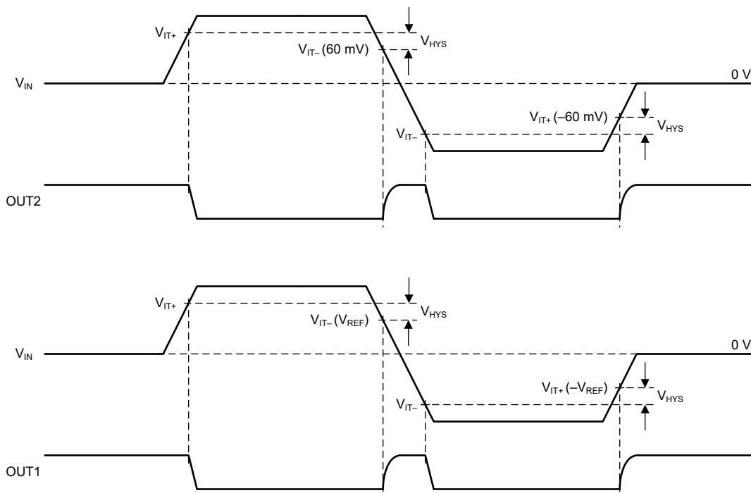
Figure 6-1. Switching Thresholds and Hysteresis
