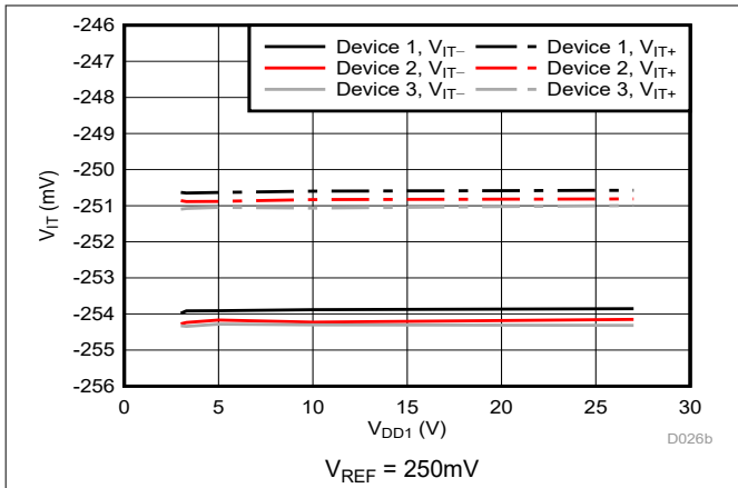
Figure 5-42. Cmp1 Trip Threshold vs Supply Voltage
