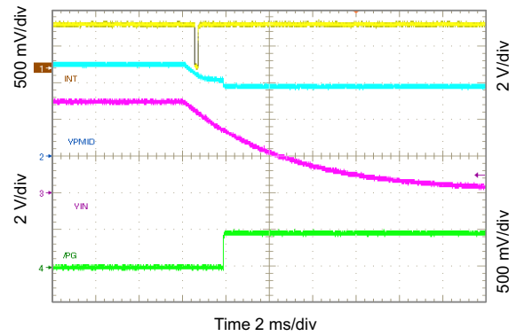
Figure 10-60. Show PG and \overline{\text{INT}} Timing ( V_{\text{IN}} Removal)
