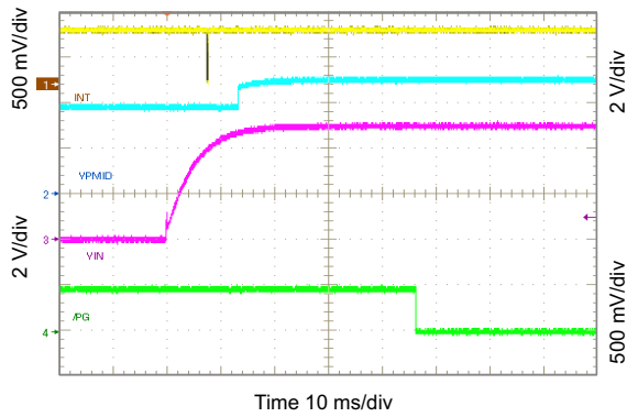
Figure 10-59. Show PG and \overline{\text{INT}} Timing ( V_{\text{IN}} Insertion)
