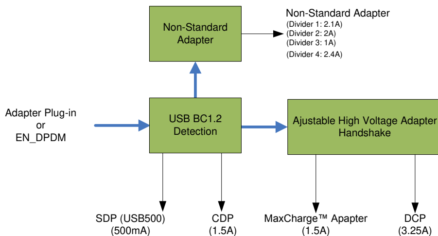
Figure 8-1. USB D+/D- Detection
