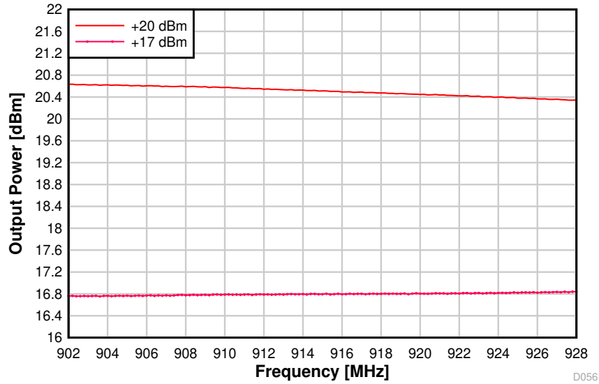
Figure 8-53. Output Power vs. Frequency (50 kbps, 915 MHz, VDDS = 3.3 V)
