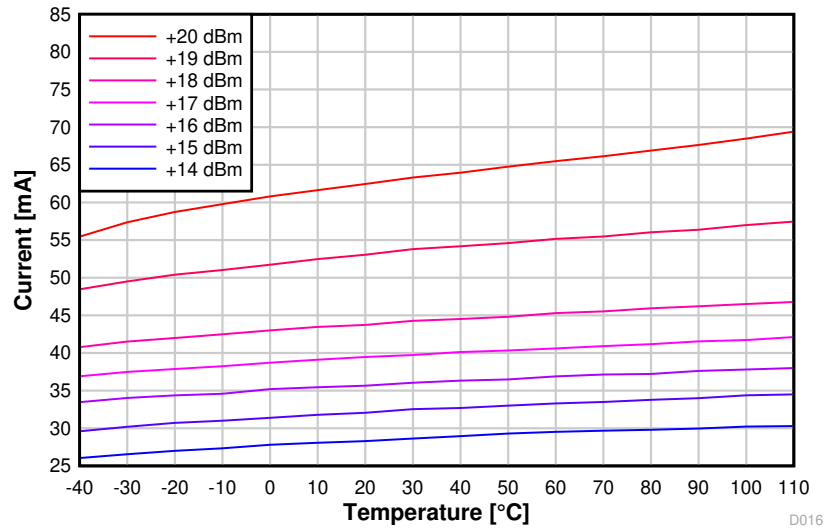
Figure 8-14. TX Current vs. Temperature (50 kbps, 915 MHz, VDDS = 3.3 V)
