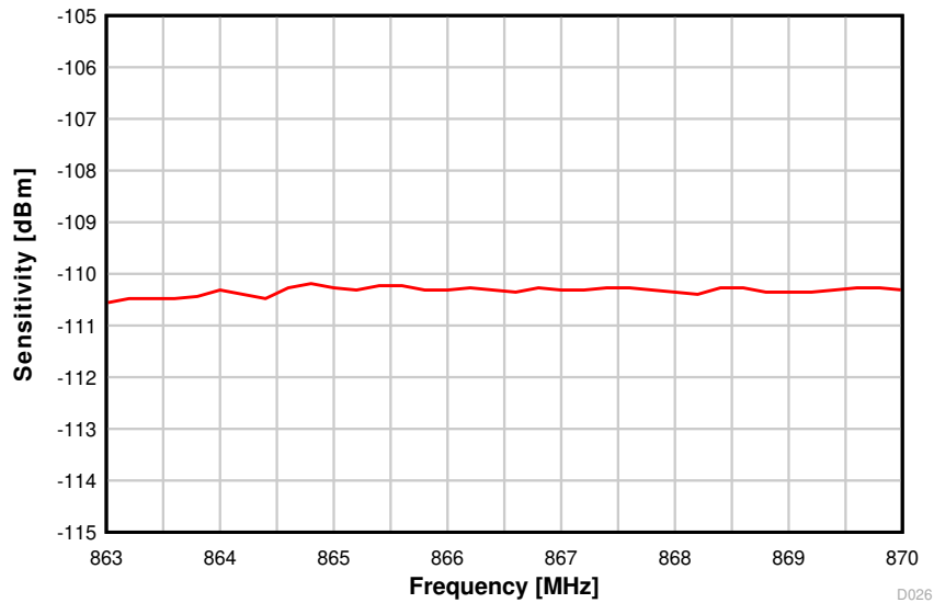
Figure 8-23. Sensitivity vs. Frequency (50 kbps, 868 MHz)
