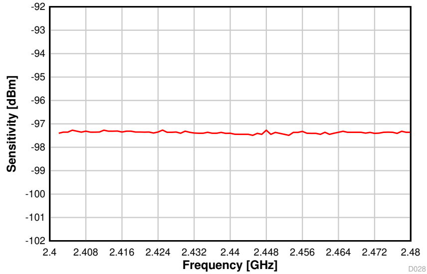
Figure 8-25. Sensitivity vs. Frequency (BLE 1 Mbps, 2.44 GHz)
