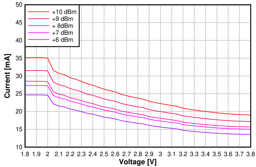
Figure 8-22. TX Current vs. Supply Voltage (VDDS) (250 kbps, 2.44 GHz, +10 dBm PA)
