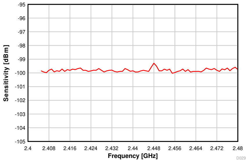
Figure 8-26. Sensitivity vs. Frequency (250 kbps, 2.44 GHz)
