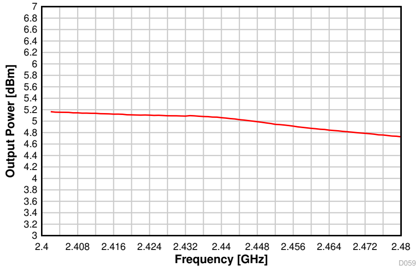
Figure 8-55. Output Power vs. Frequency (BLE 1 Mbps, 2.44 GHz, +5 dBm)
