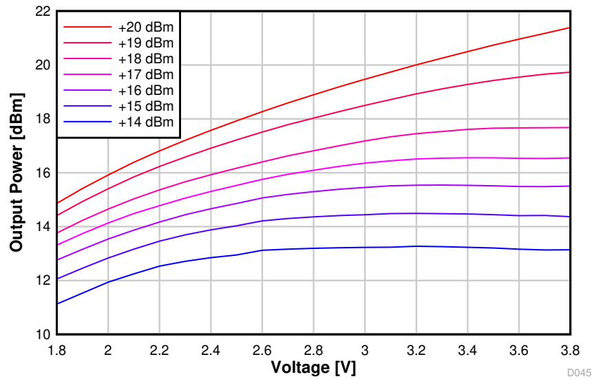
Figure 8-46. Output Power vs. Supply Voltage (VDDS) (50 kbps, 915 MHz)
