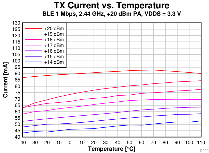
Figure 8-16. TX Current vs. Temperature (BLE 1 Mbps, 2.44 GHz, VDDS = 3.3 V)
