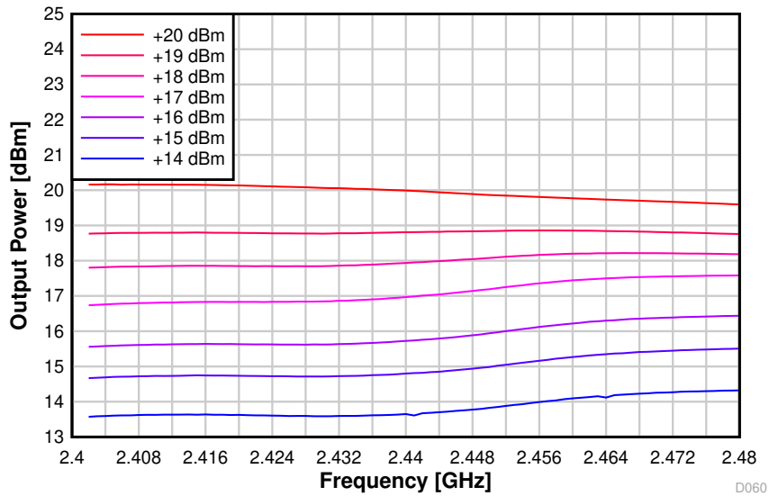
Figure 8-56. Output Power vs. Frequency (BLE 1 Mbps, 2.44 GHz, +20 dBm PA)
