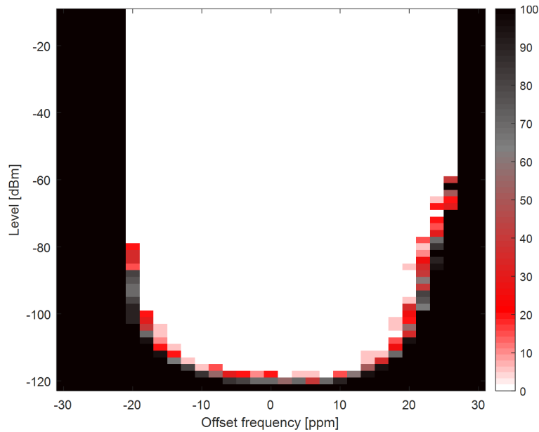
Figure 8-38. Narrowband, WMBUS N-MODE, 2.4 kbps, 169 MHz
