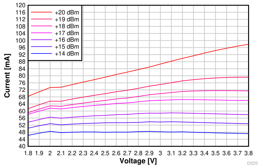
Figure 8-21. TX Current vs. Supply Voltage (VDDS) (BLE 1 Mbps, 2.44 GHz, +20 dBm PA)
