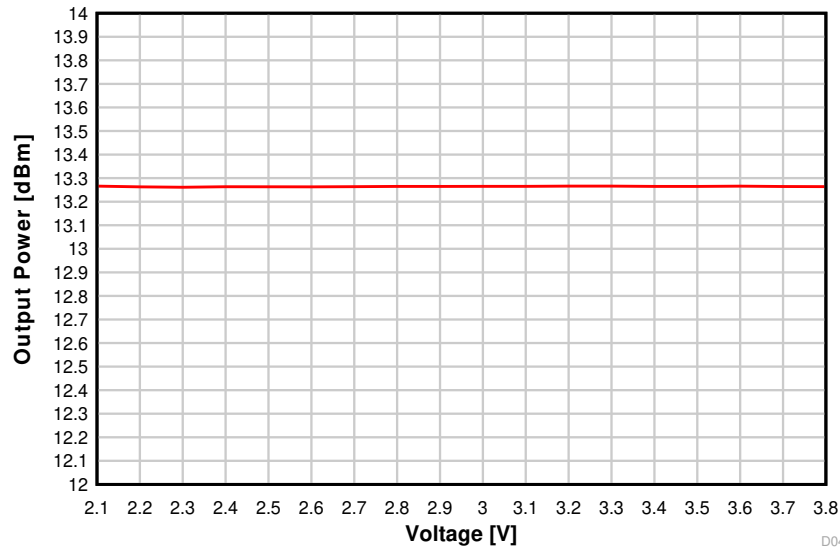
Figure 8-45. Output Power vs. Supply Voltage (VDDS) (50 kbps, 868.3 MHz)
