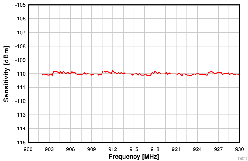
Figure 8-24. Sensitivity vs. Frequency (50 kbps, 915 MHz)
