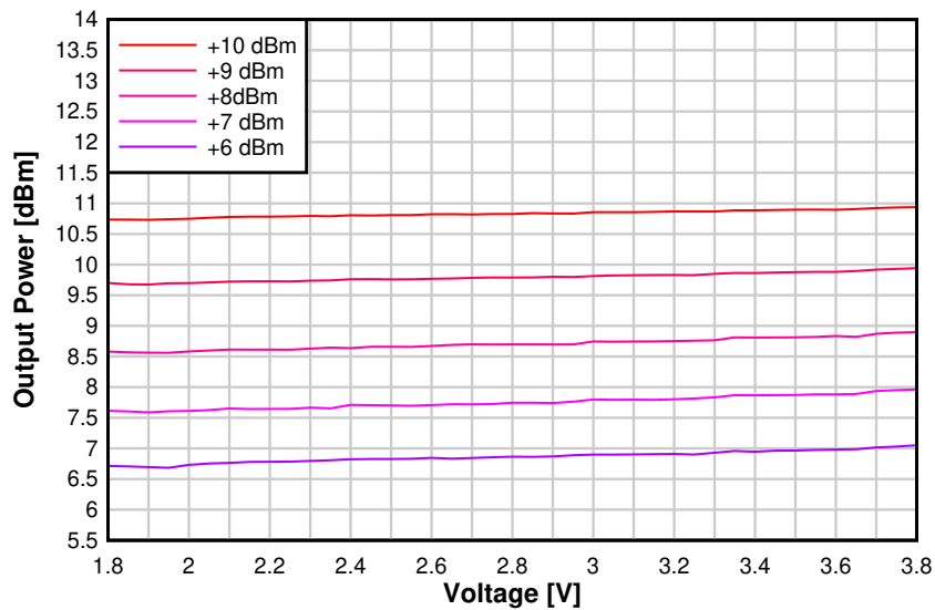
Figure 8-50. Output Power vs. Supply Voltage (VDD5) (2.44 GHz, +10 dBm PA)
