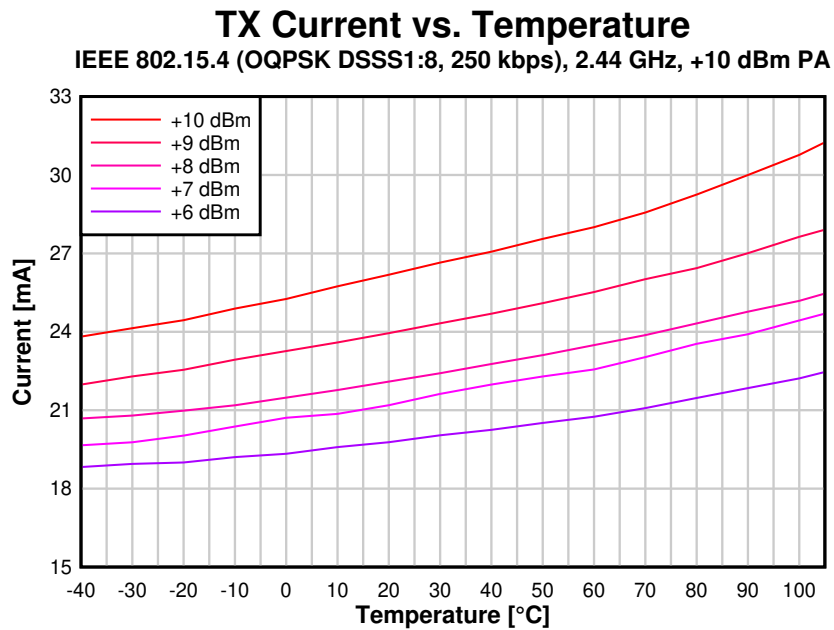
Figure 8-17. TX Current vs. Temperature (250 kbps, 2.44 GHz, +10 dBm PA)
