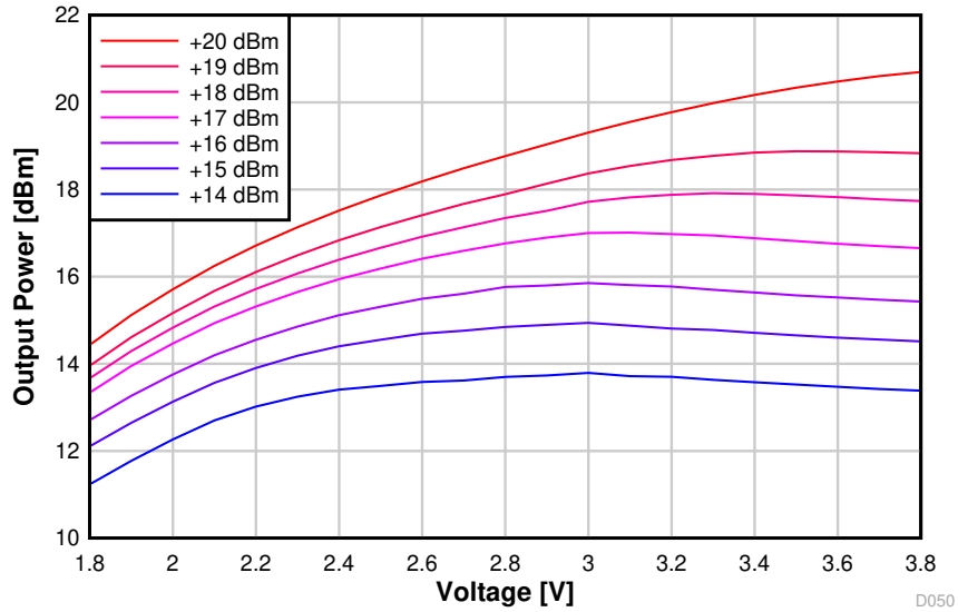
Figure 8-49. Output Power vs. Supply Voltage (VDD5) (BLE 1 Mbps, 2.44 GHz, +20 dBm PA)
