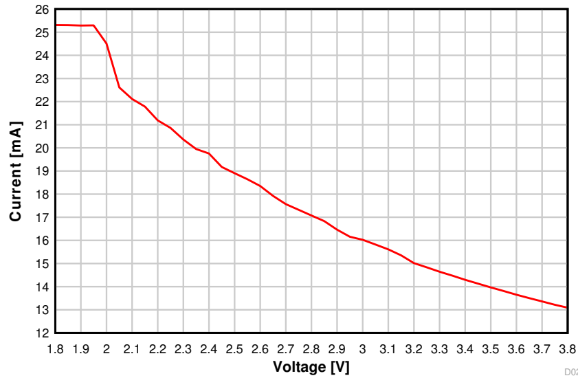
Figure 8-18. TX Current vs. Supply Voltage (VDDS) (50 kbps, 868.3 MHz)
