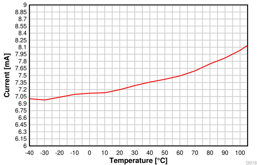
Figure 8-15. TX Current vs. Temperature (BLE 1 Mbps, 2.44 GHz)
