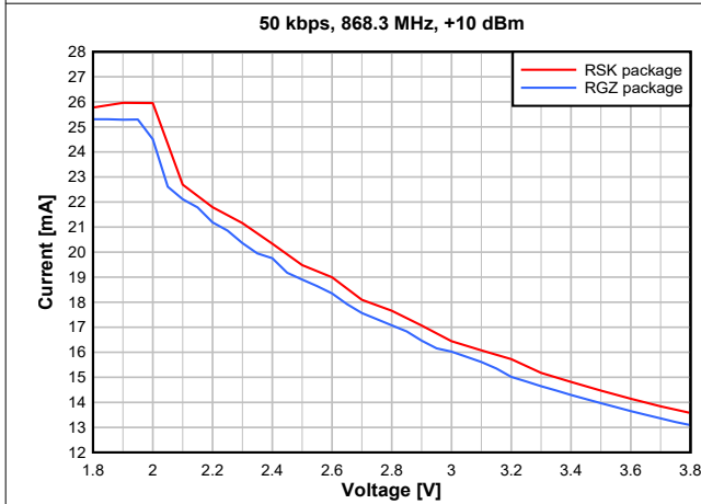
Figure 7-12. TX Current vs. Supply Voltage (VDDS) (50kbps, 868.3MHz)
