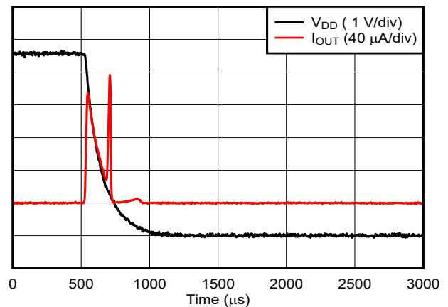
DAC at mid scale ( 0\ \mu\text{A} ) Figure 6-46. Current Output Power-Off Glitch
