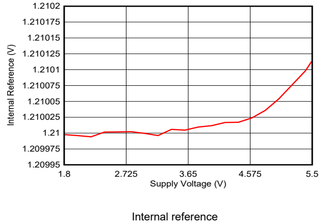
Figure 6-55. Internal Reference vs Supply Voltage
