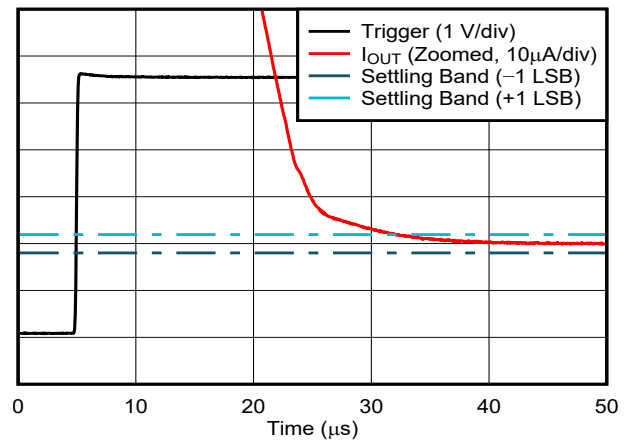
Figure 6-44. Current Output Settling Time: Falling Edge (1/4 to 3/4 scale)
