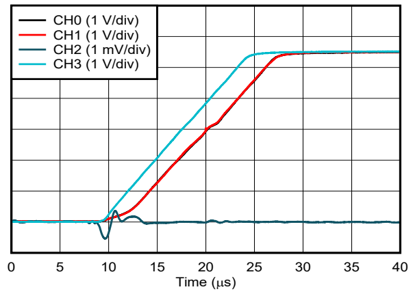
Channel 2 is resident, all other channels are interferers Figure 6-25. Voltage Output Channel-to-Channel Crosstalk
