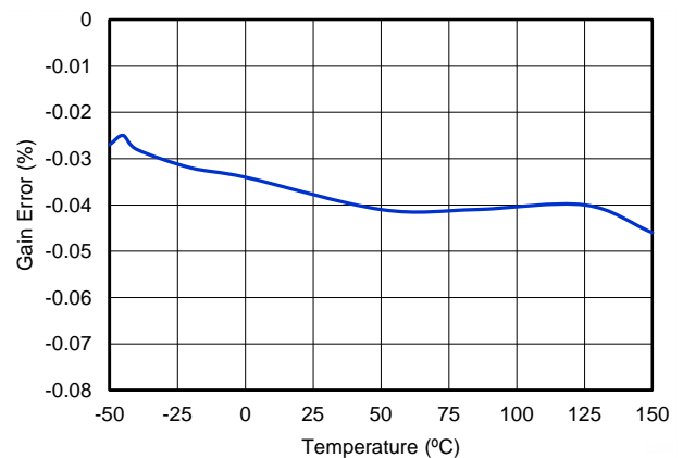
Figure 24. DIFFERENTIAL AMPLIFIER GAIN ERROR vs TEMPERATURE
