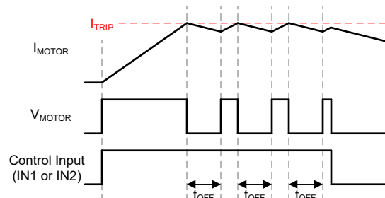
Figure 8-5. Off-Time Current-Regulation
