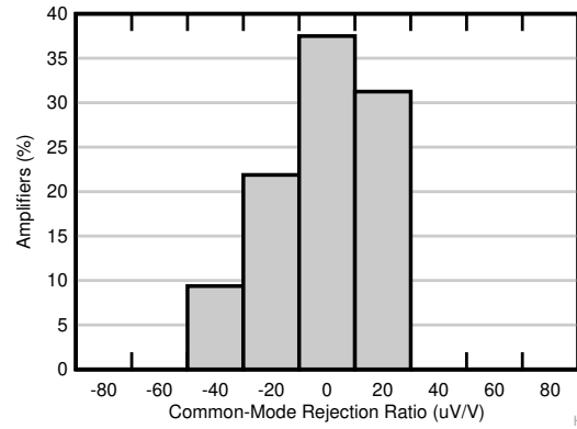
Figure 6-8. Typical Distribution of Output Referred CMRR
