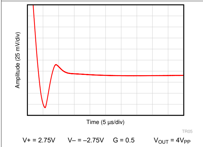
Figure 6-53. Large Signal Settling Time (Falling Edge)
