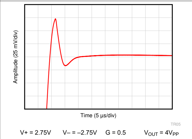
Figure 6-54. Large Signal Settling Time (Rising Edge)
