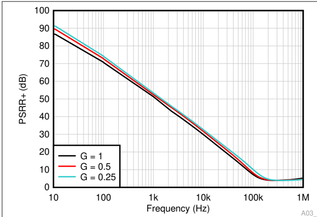
Figure 6-37. PSRR+ (Referred to Output) vs Frequency
