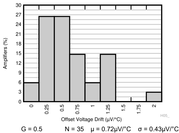
Figure 6-5. Typical Distribution of Output Referred Offset Drift
