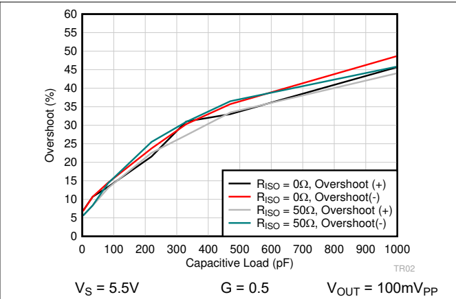
Figure 6-62. Small-Signal Overshoot vs Capacitive Load
