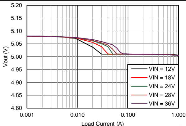
Figure 61. Output Voltage Regulation
