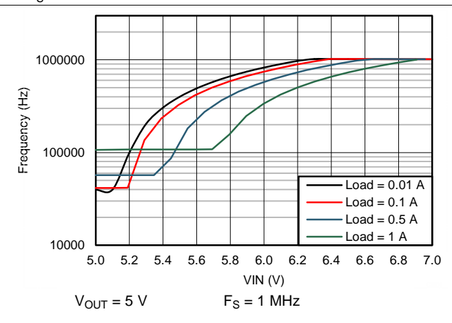
Figure 20. Switching Frequency vs V_{IN} in Dropout Operation
