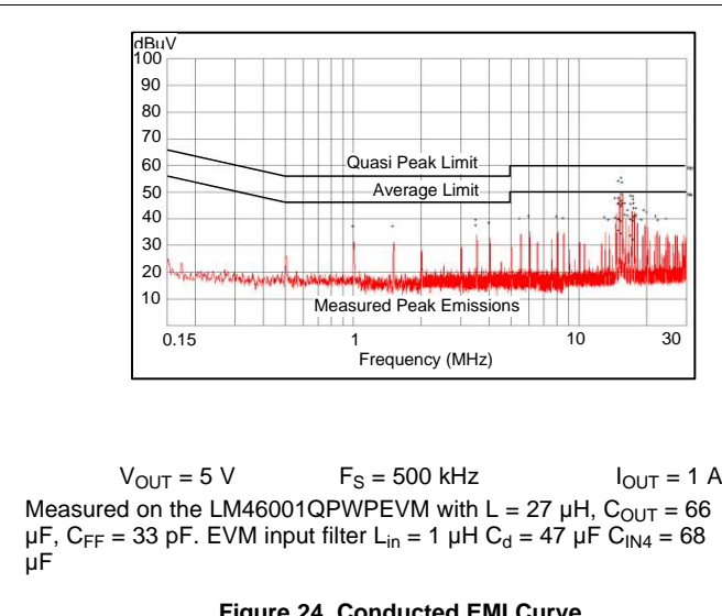
Figure 24. Conducted EMI Curve
