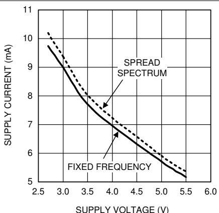
Figure 17. Supply Current vs Supply Voltage PV_1 = 4.8\text{ V}
