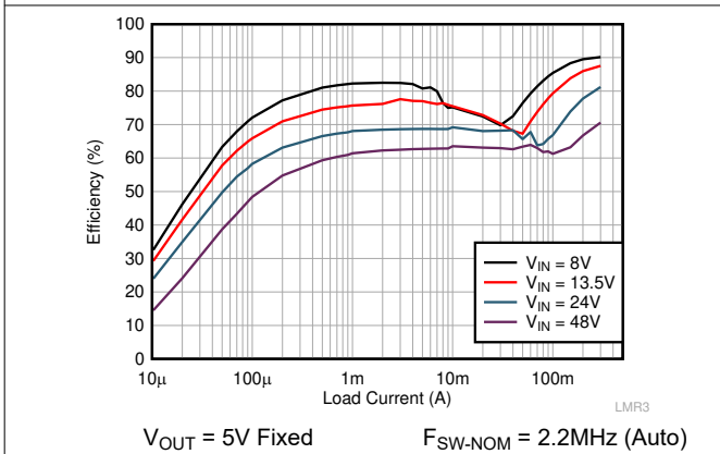
Figure 6-3. Efficiency 5V Output, Auto Mode
