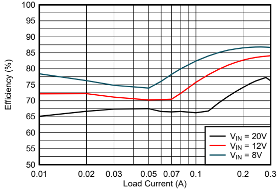
Figure 8-10. Efficiency
