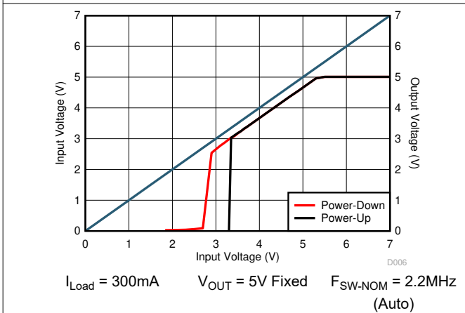
Figure 6-5. Dropout at Power-Up and Power-Down
