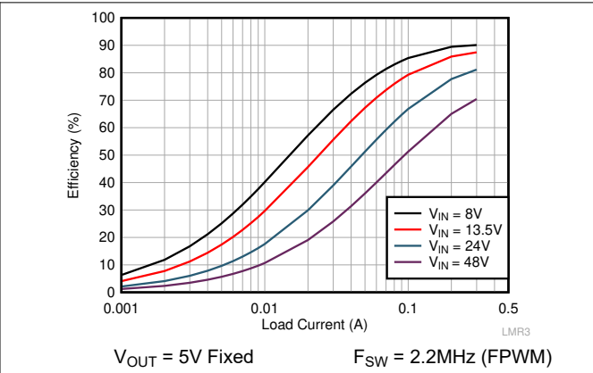
Figure 6-2. Efficiency 5V Output, FPWM
