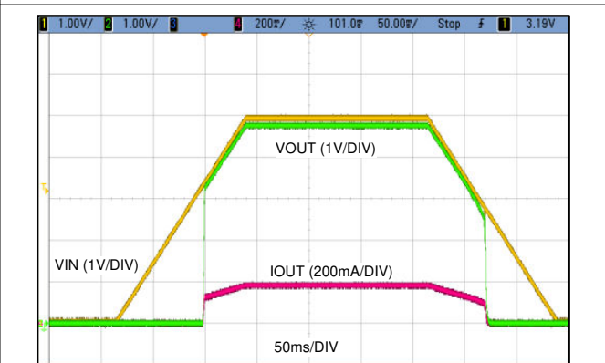
Figure 6-6. Typical Start-up and Shutdown at V_{OUT} = 5\text{V}
