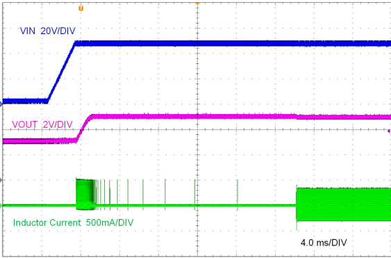
LMR38015-Q1 V_{OUT} = 5\text{ V} No Load Bias to 3 V
