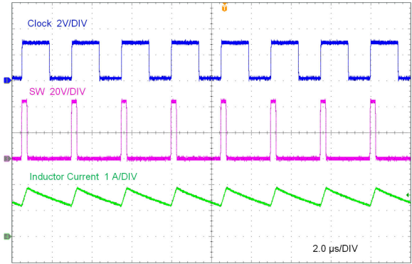
LMR38015-Q1 V_{OUT} = 5\text{ V} 400 kHz
