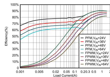
Efficiency vs Output Current V_{OUT} = 5\text{ V} , 400 kHz
