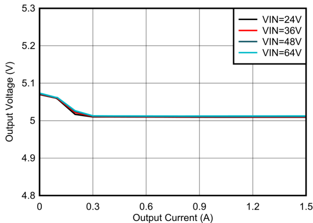
LMR38015-Q1 V_{OUT} = 5\text{ V} 400 kHz PFM Version
