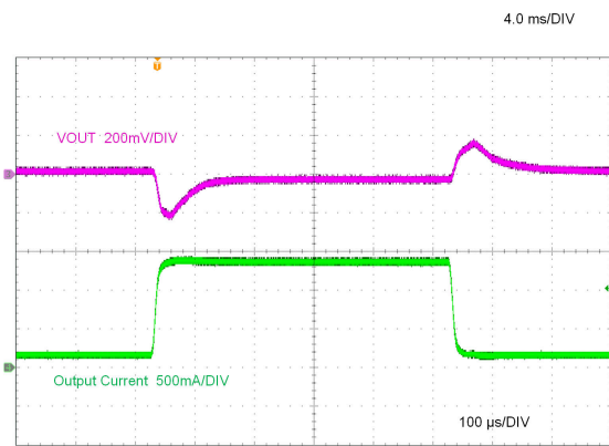
LMR38015-Q1 V_{OUT} = 5\text{ V} 400 kHz (AC Coupled)
