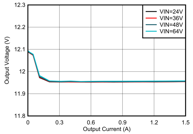
LMR38015-Q1 V_{OUT} = 12\text{ V} 400 kHz PFM Version
