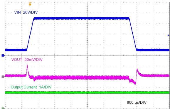
LMR38015-Q1 V_{OUT} = 5\text{ V} 400 kHz (AC Coupled)
