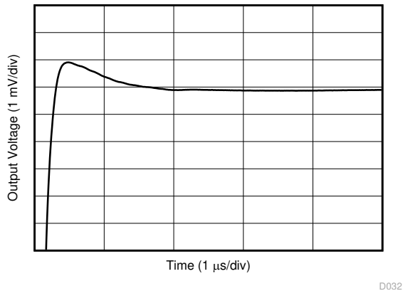
Figure 5-27. Large-Signal Settling Time (Positive)
