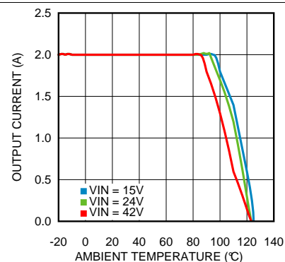
Figure 48. Thermal Derating V OUT = 12 V, R θJA = 16°C/W
