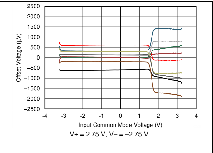
Figure 2. Offset Voltage vs Common-Mode Voltage
