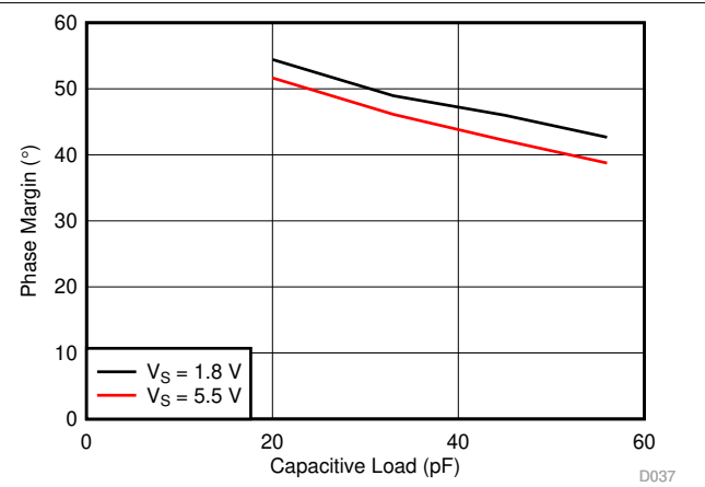
Figure 7-38. Phase Margin vs Capacitive Load
