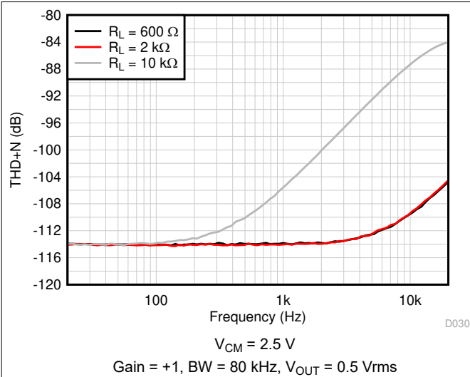
Figure 7-69. THD + N vs Frequency
