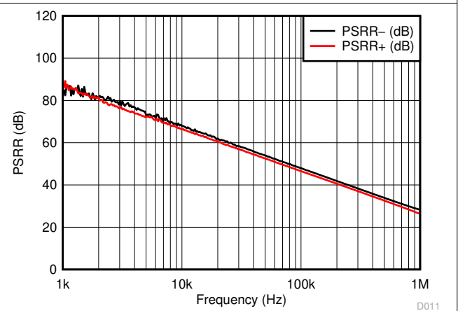
Figure 7-12. PSRR vs Frequency (Referred to Input)
