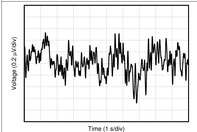
Figure 7-49. 0.1-Hz to 10-Hz Flicker Noise
