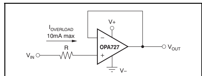
Figure 29. Input Current Protection for Voltages Exceeding the Supply Voltage
